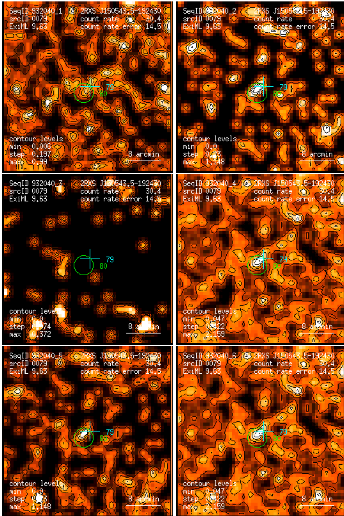
Figure 79: RASS 932040: detection 0079: band rate images, Gaussian filter: (1) PSPC channels 11 – 41, (2) 52 – 90, (3) 91 – 201, (4) 11 – 235, (5) 52 – 201, (6) 11 – 201. Broad band rates in counts/ks. Band rate contour levels in counts/ks/arcmin 2 .
