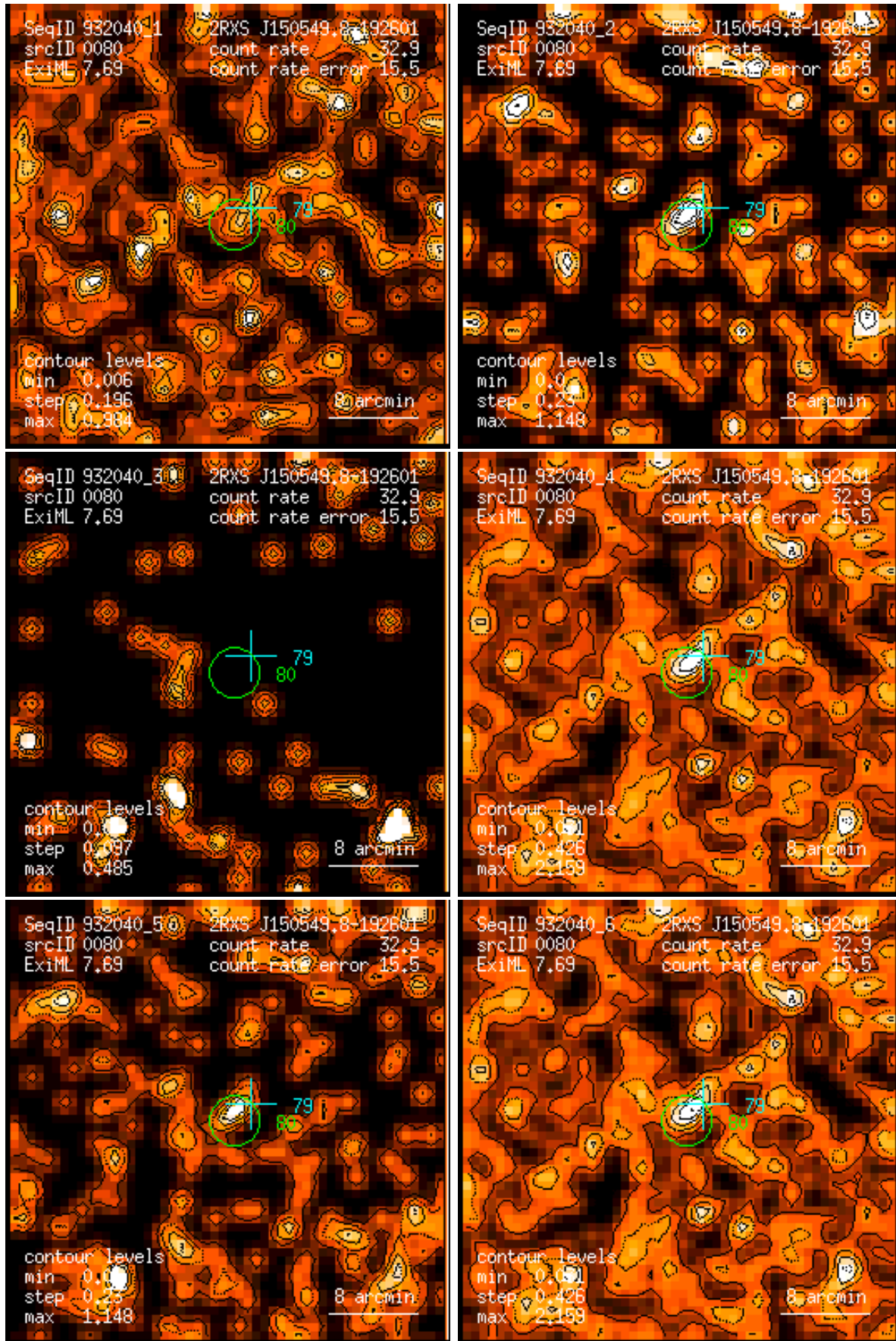
Figure 80: RASS 932040: detection 0080: band rate images, Gaussian filter: (1) PSPC channels 11 – 41, (2) 52 – 90, (3) 91 – 201, (4) 11 – 235, (5) 52 – 201, (6) 11 – 201. Broad band rates in counts/ks. Band rate contour levels in counts/ks/arcmin 2 .
