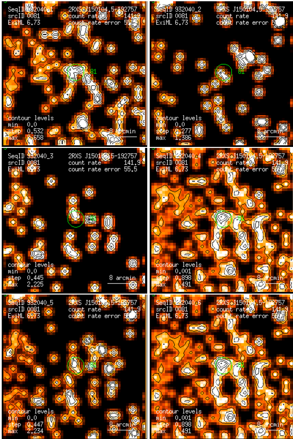
Figure 81: RASS 932040: detection 0081: band rate images, Gaussian filter: (1) PSPC channels 11 – 41, (2) 52 – 90, (3) 91 – 201, (4) 11 – 235, (5) 52 – 201, (6) 11 – 201. Broad band rates in counts/ks. Band rate contour levels in counts/ks/arcmin 2 .
