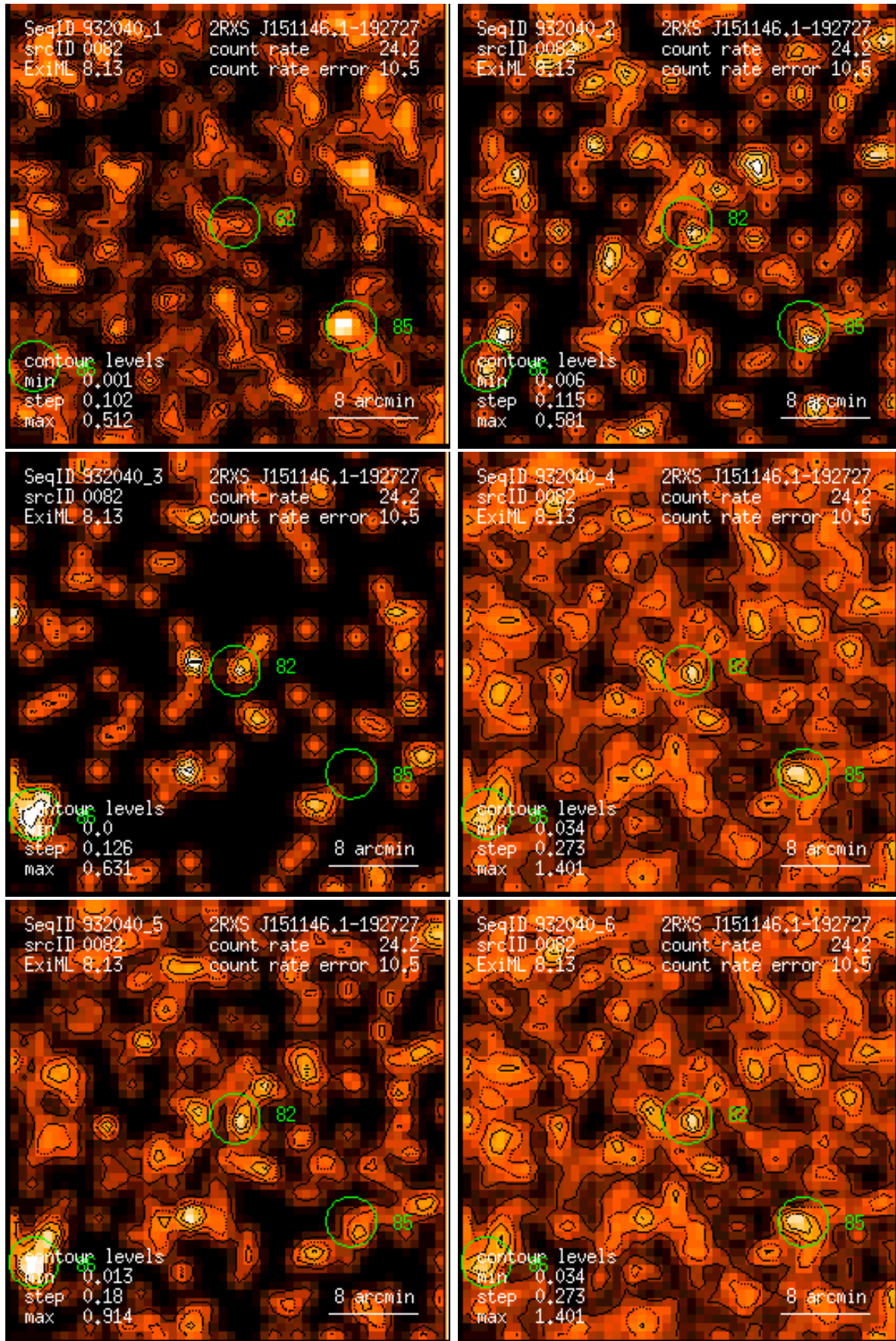
Figure 82: RASS 932040: detection 0082: band rate images, Gaussian filter: (1) PSPC channels 11 – 41, (2) 52 – 90, (3) 91 – 201, (4) 11 – 235, (5) 52 – 201, (6) 11 – 201. Broad band rates in counts/ks. Band rate contour levels in counts/ks/arcmin 2 .
