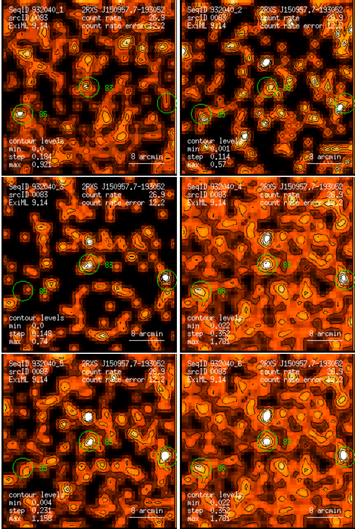
Figure 83: RASS 932040: detection 0083: band rate images, Gaussian filter: (1) PSPC channels 11 – 41, (2) 52 – 90, (3) 91 – 201, (4) 11 – 235, (5) 52 – 201, (6) 11 – 201. Broad band rates in counts/ks. Band rate contour levels in counts/ks/arcmin 2 .
