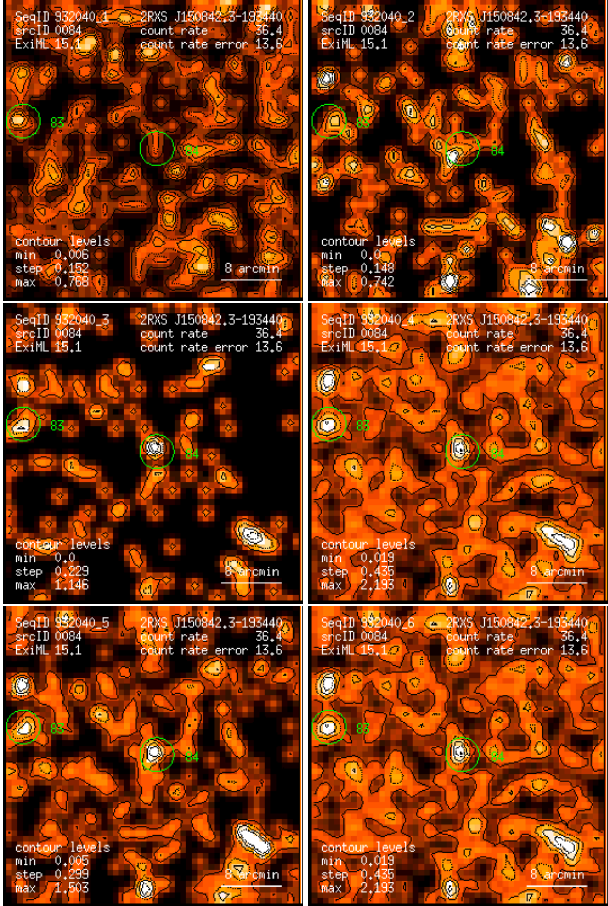
Figure 84: RASS 932040: detection 0084: band rate images, Gaussian filter: (1) PSPC channels 11 – 41, (2) 52 – 90, (3) 91 – 201, (4) 11 – 235, (5) 52 – 201, (6) 11 – 201. Broad band rates in counts/ks. Band rate contour levels in counts/ks/arcmin 2 .
