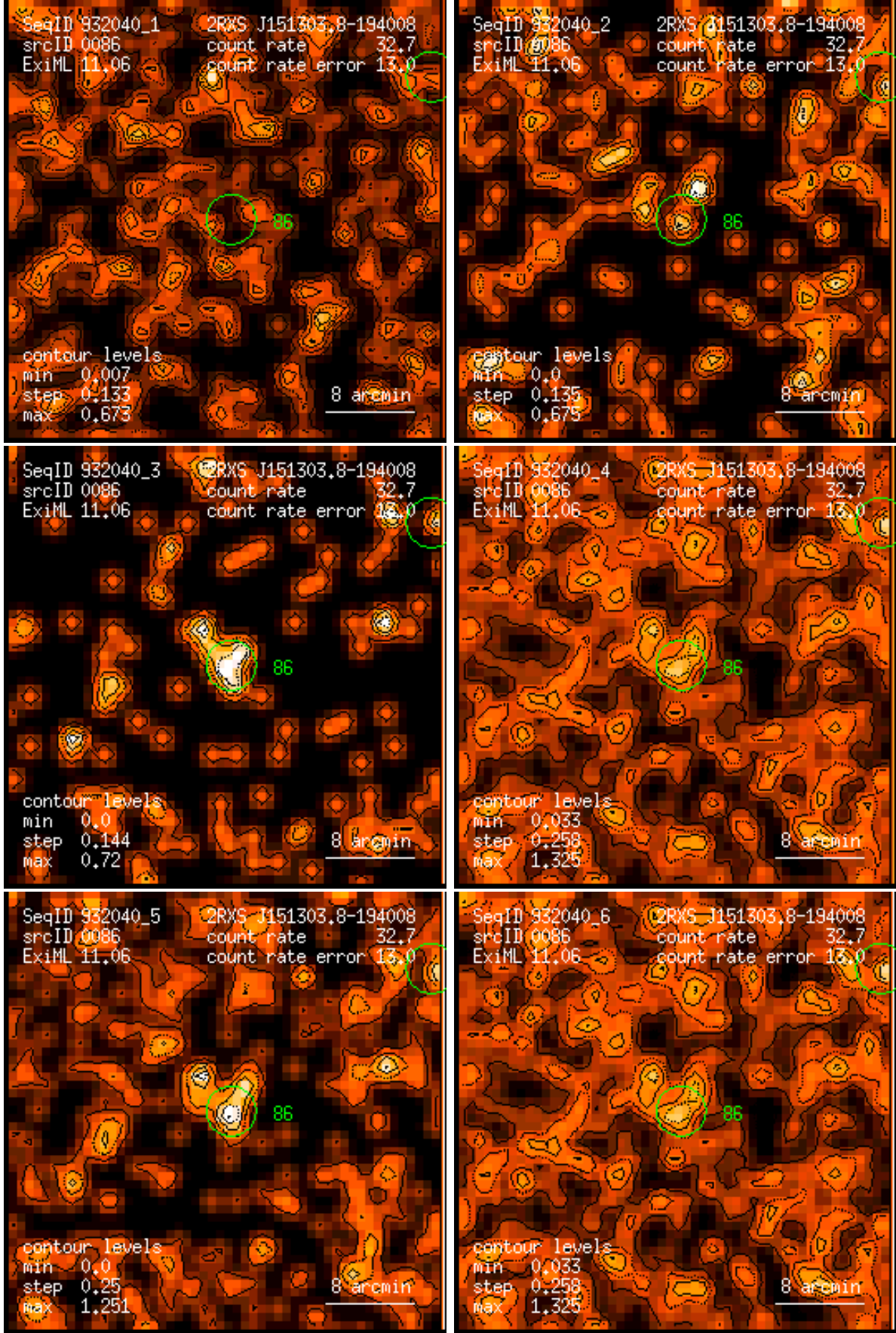
Figure 86: RASS 932040: detection 0086: band rate images, Gaussian filter: (1) PSPC channels 11 – 41, (2) 52 – 90, (3) 91 – 201, (4) 11 – 235, (5) 52 – 201, (6) 11 – 201. Broad band rates in counts/ks. Band rate contour levels in counts/ks/arcmin 2 .
