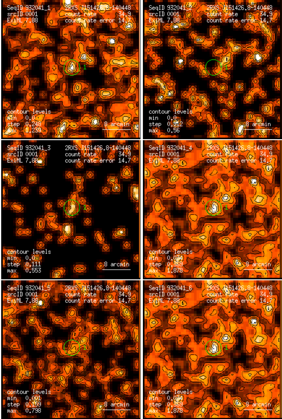
Figure 1: RASS 932041: detection 0001: band rate images, Gaussian filter: (1) PSPC channels 11 – 41, (2) 52 – 90, (3) 91 – 201, (4) 11 – 235, (5) 52 – 201, (6) 11 – 201. Broad band rates in counts/ks. Band rate contour levels in counts/ks/arcmin 2 .
