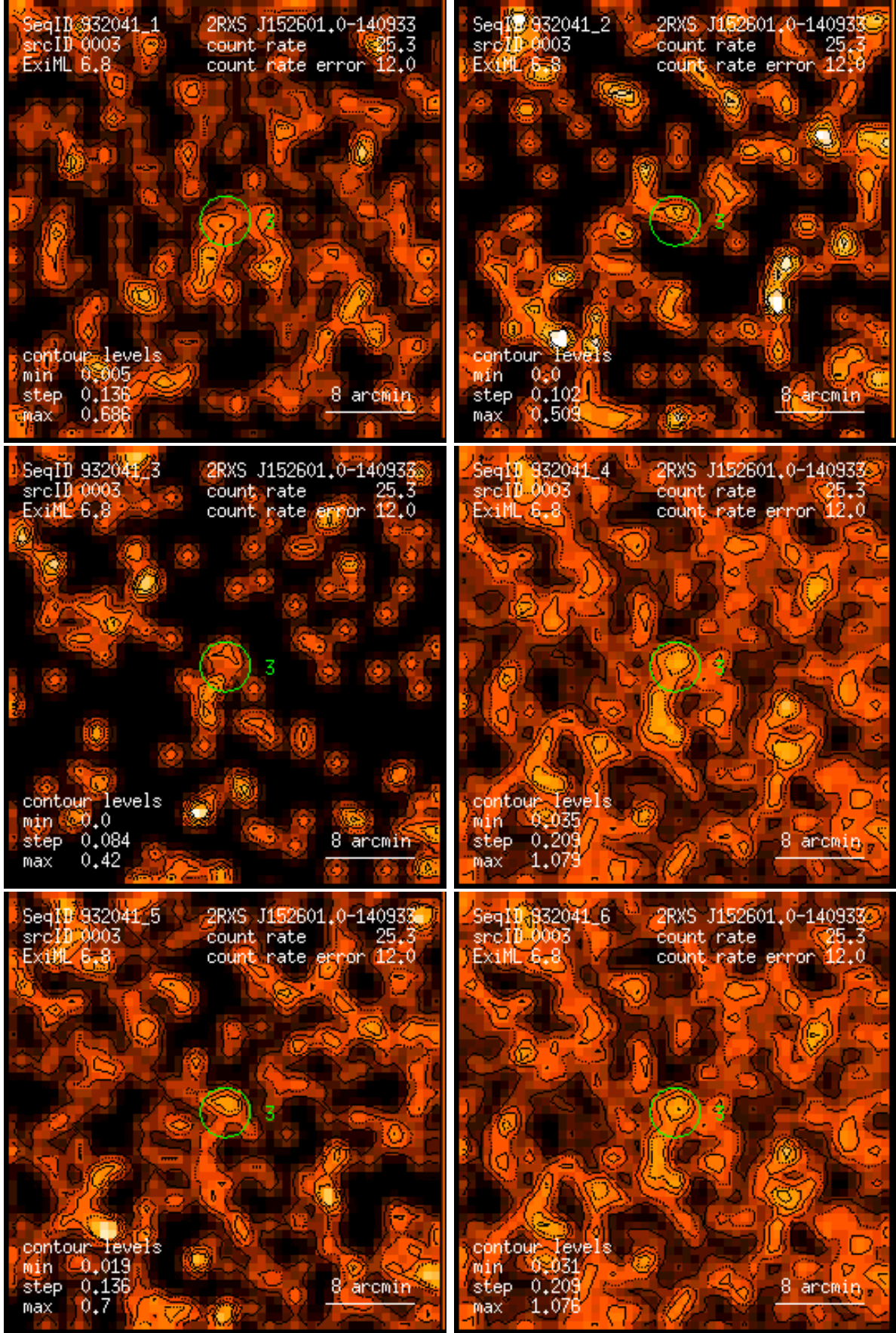
Figure 3: RASS 932041: detection 0003: band rate images, Gaussian filter: (1) PSPC channels 11 – 41, (2) 52 – 90, (3) 91 – 201, (4) 11 – 235, (5) 52 – 201, (6) 11 – 201. Broad band rates in counts/ks. Band rate contour levels in counts/ks/arcmin 2 .
