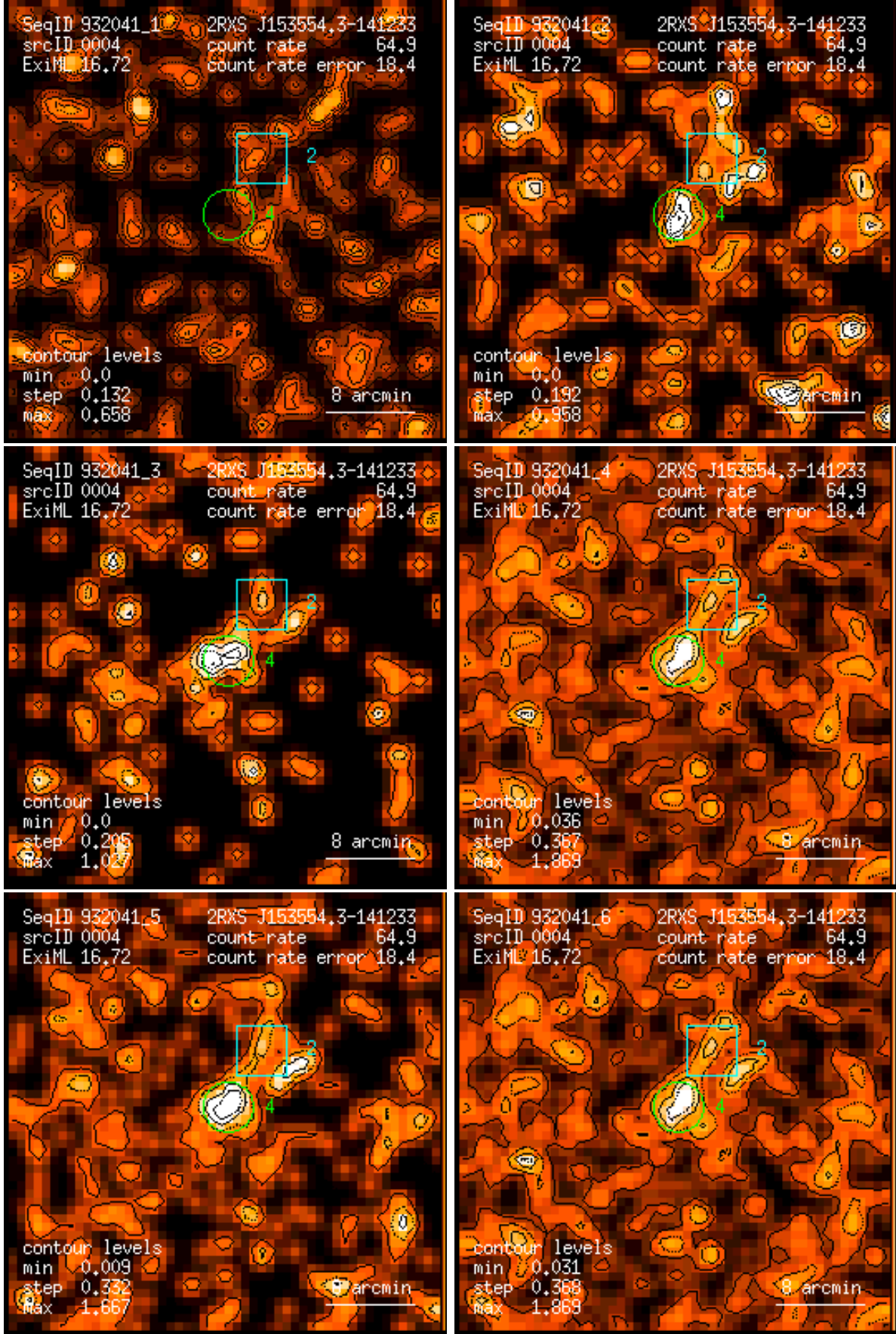
Figure 4: RASS 932041: detection 0004: band rate images, Gaussian filter: (1) PSPC channels 11 – 41, (2) 52 – 90, (3) 91 – 201, (4) 11 – 235, (5) 52 – 201, (6) 11 – 201. Broad band rates in counts/ks. Band rate contour levels in counts/ks/arcmin 2 .
