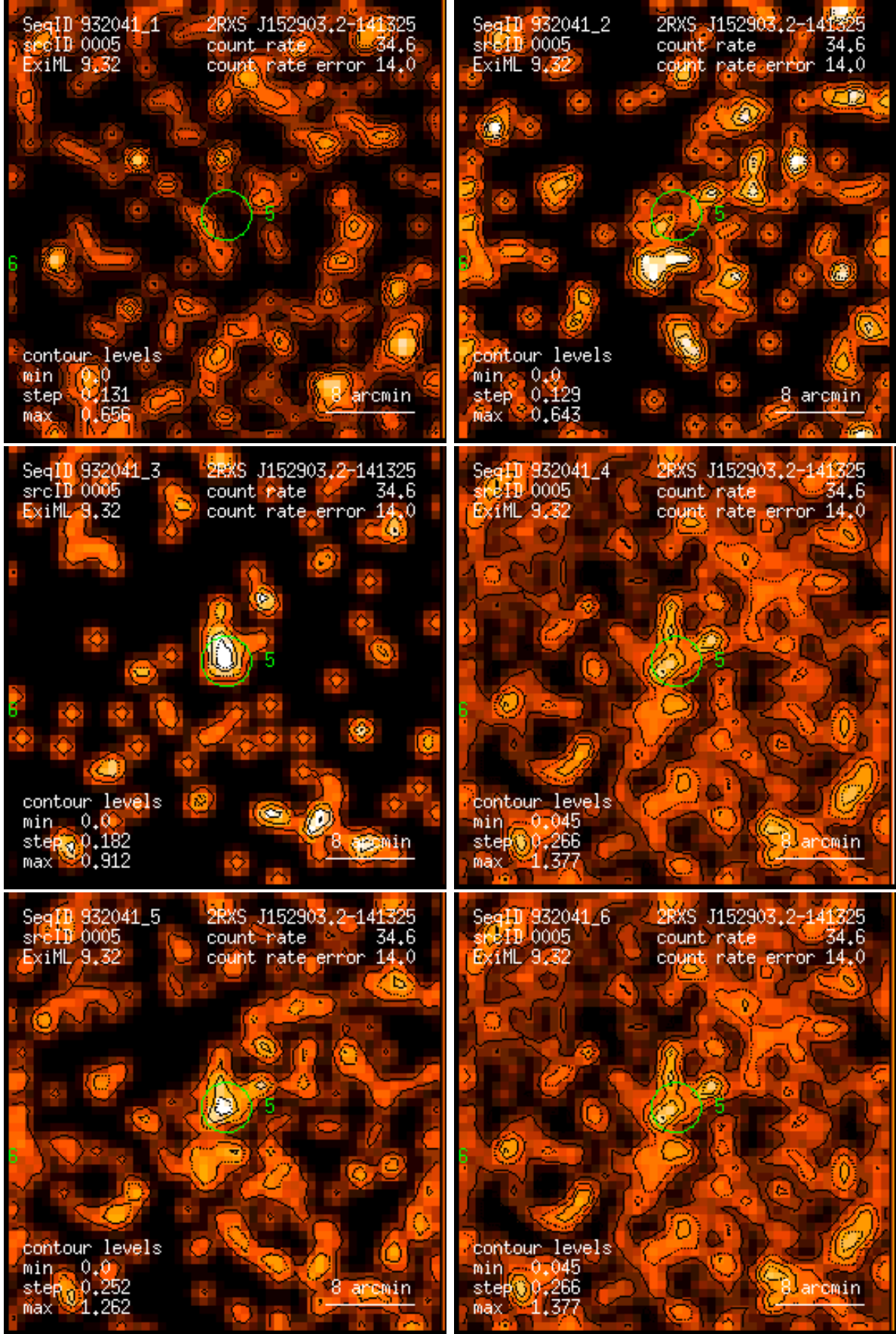
Figure 5: RASS 932041: detection 0005: band rate images, Gaussian filter: (1) PSPC channels 11 – 41, (2) 52 – 90, (3) 91 – 201, (4) 11 – 235, (5) 52 – 201, (6) 11 – 201. Broad band rates in counts/ks. Band rate contour levels in counts/ks/arcmin 2 .
