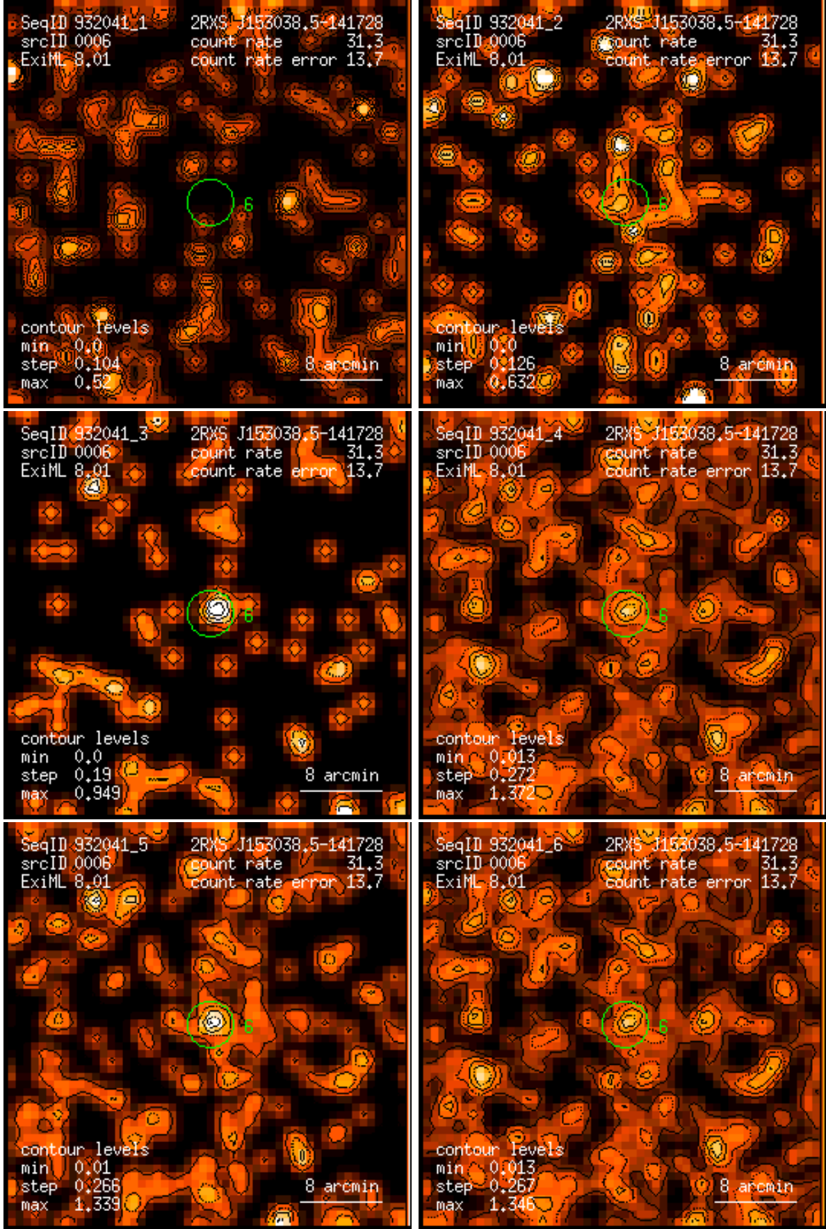
Figure 6: RASS 932041: detection 0006: band rate images, Gaussian filter: (1) PSPC channels 11 – 41, (2) 52 – 90, (3) 91 – 201, (4) 11 – 235, (5) 52 – 201, (6) 11 – 201. Broad band rates in counts/ks. Band rate contour levels in counts/ks/arcmin 2 .
