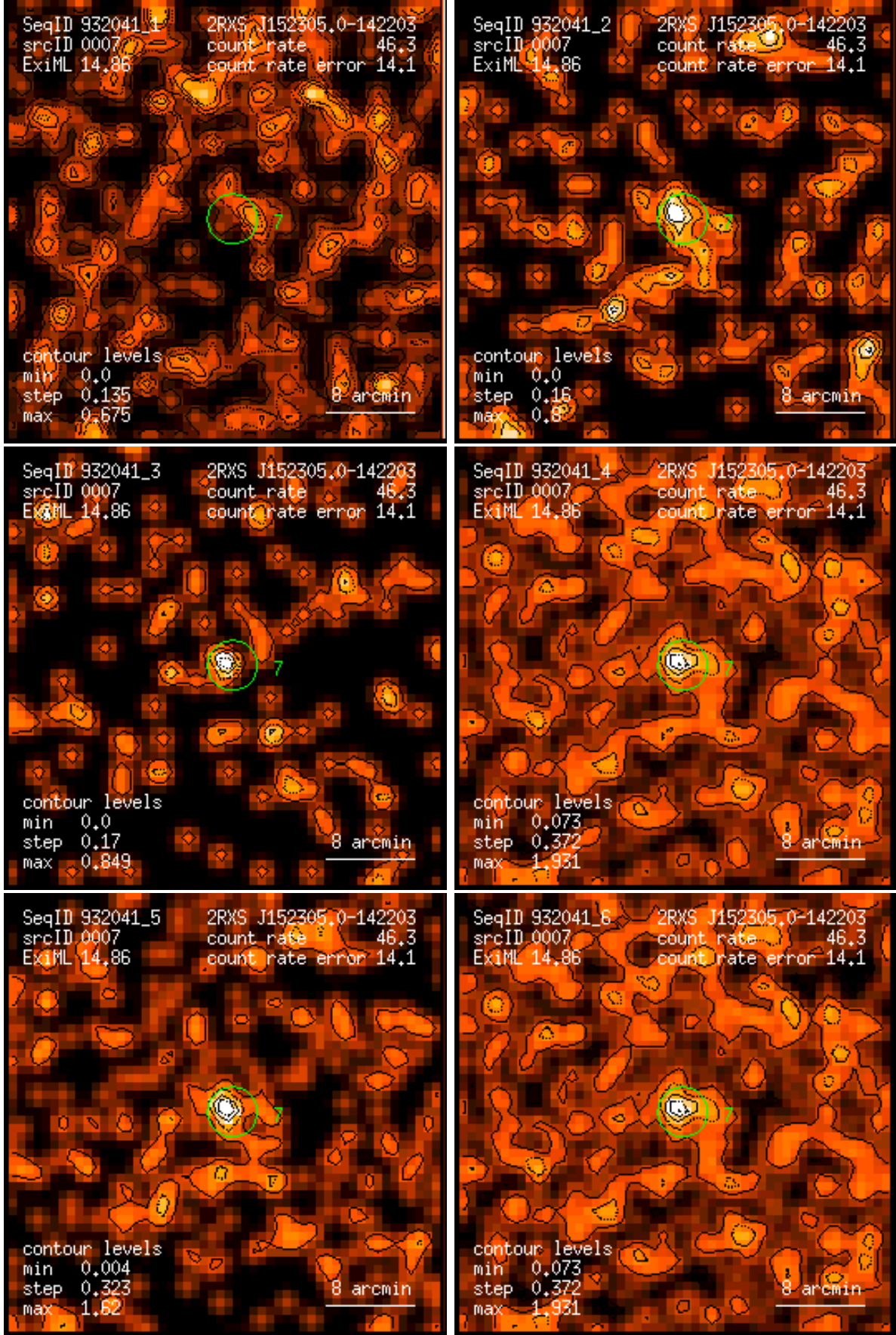
Figure 7: RASS 932041: detection 0007: band rate images, Gaussian filter: (1) PSPC channels 11 – 41, (2) 52 – 90, (3) 91 – 201, (4) 11 – 235, (5) 52 – 201, (6) 11 – 201. Broad band rates in counts/ks. Band rate contour levels in counts/ks/arcmin 2 .
