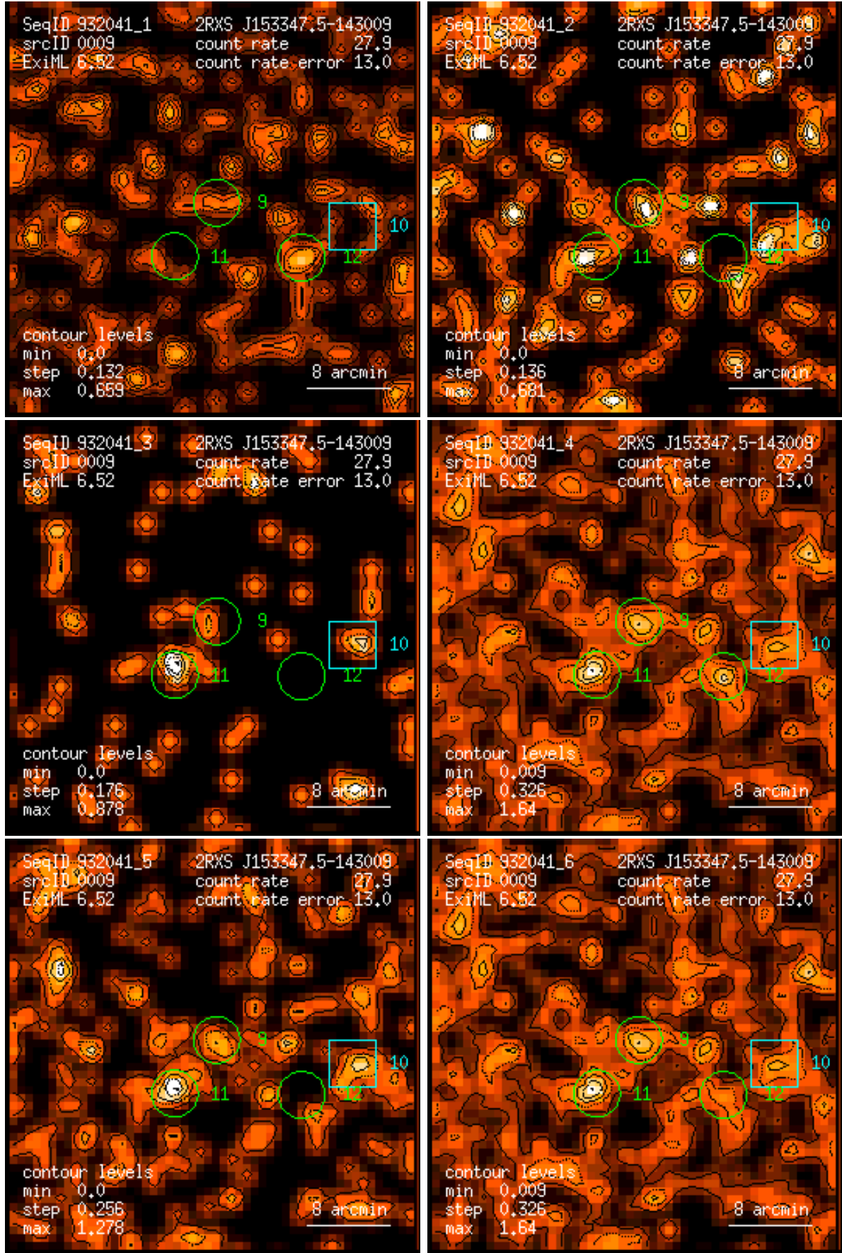
Figure 9: RASS 932041: detection 0009: band rate images, Gaussian filter: (1) PSPC channels 11 – 41, (2) 52 – 90, (3) 91 – 201, (4) 11 – 235, (5) 52 – 201, (6) 11 – 201. Broad band rates in counts/ks. Band rate contour levels in counts/ks/arcmin 2 .
