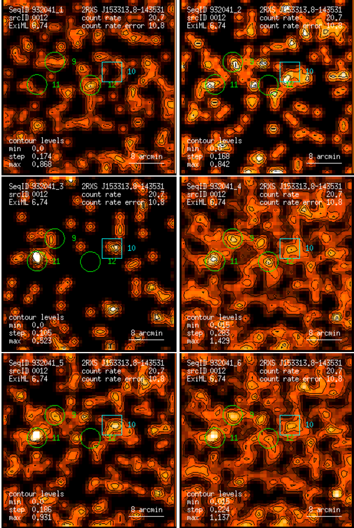
Figure 12: RASS 932041: detection 0012: band rate images, Gaussian filter: (1) PSPC channels 11 – 41, (2) 52 – 90, (3) 91 – 201, (4) 11 – 235, (5) 52 – 201, (6) 11 – 201. Broad band rates in counts/ks. Band rate contour levels in counts/ks/arcmin 2 .
