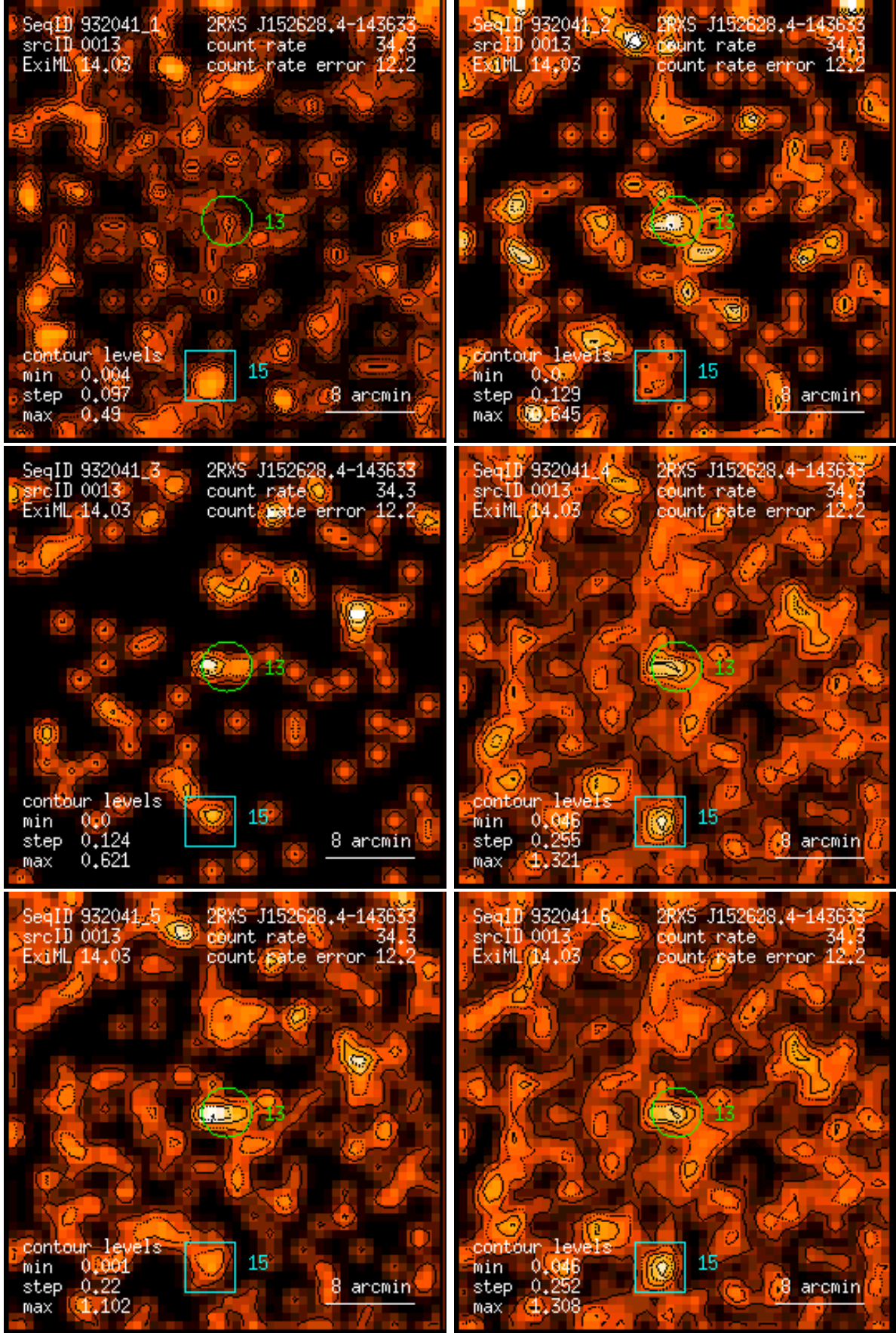
Figure 13: RASS 932041: detection 0013: band rate images, Gaussian filter: (1) PSPC channels 11 – 41, (2) 52 – 90, (3) 91 – 201, (4) 11 – 235, (5) 52 – 201, (6) 11 – 201. Broad band rates in counts/ks. Band rate contour levels in counts/ks/arcmin 2 .
