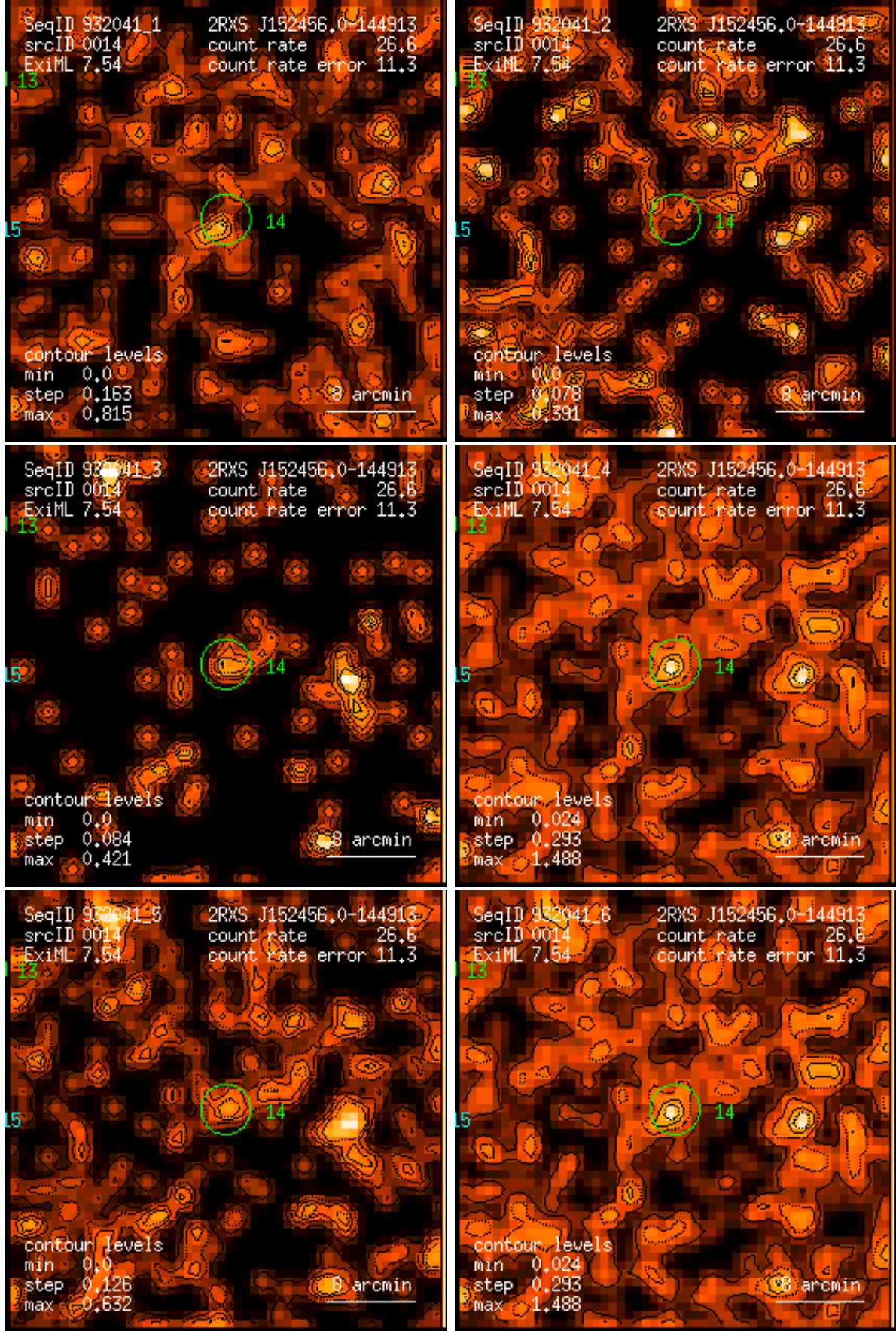
Figure 14: RASS 932041: detection 0014: band rate images, Gaussian filter: (1) PSPC channels 11 – 41, (2) 52 – 90, (3) 91 – 201, (4) 11 – 235, (5) 52 – 201, (6) 11 – 201. Broad band rates in counts/ks. Band rate contour levels in counts/ks/arcmin 2 .
