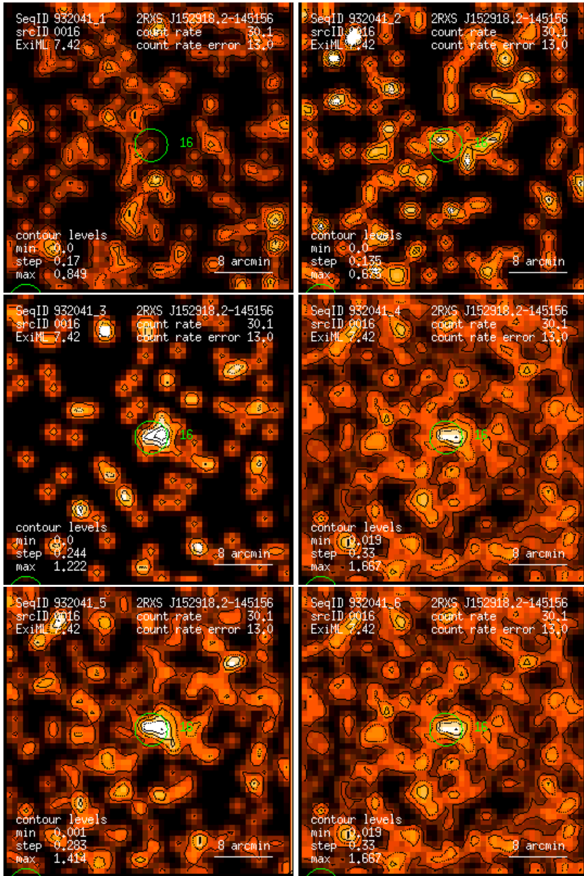
Figure 16: RASS 932041: detection 0016: band rate images, Gaussian filter: (1) PSPC channels 11 – 41, (2) 52 – 90, (3) 91 – 201, (4) 11 – 235, (5) 52 – 201, (6) 11 – 201. Broad band rates in counts/ks. Band rate contour levels in counts/ks/arcmin 2 .
