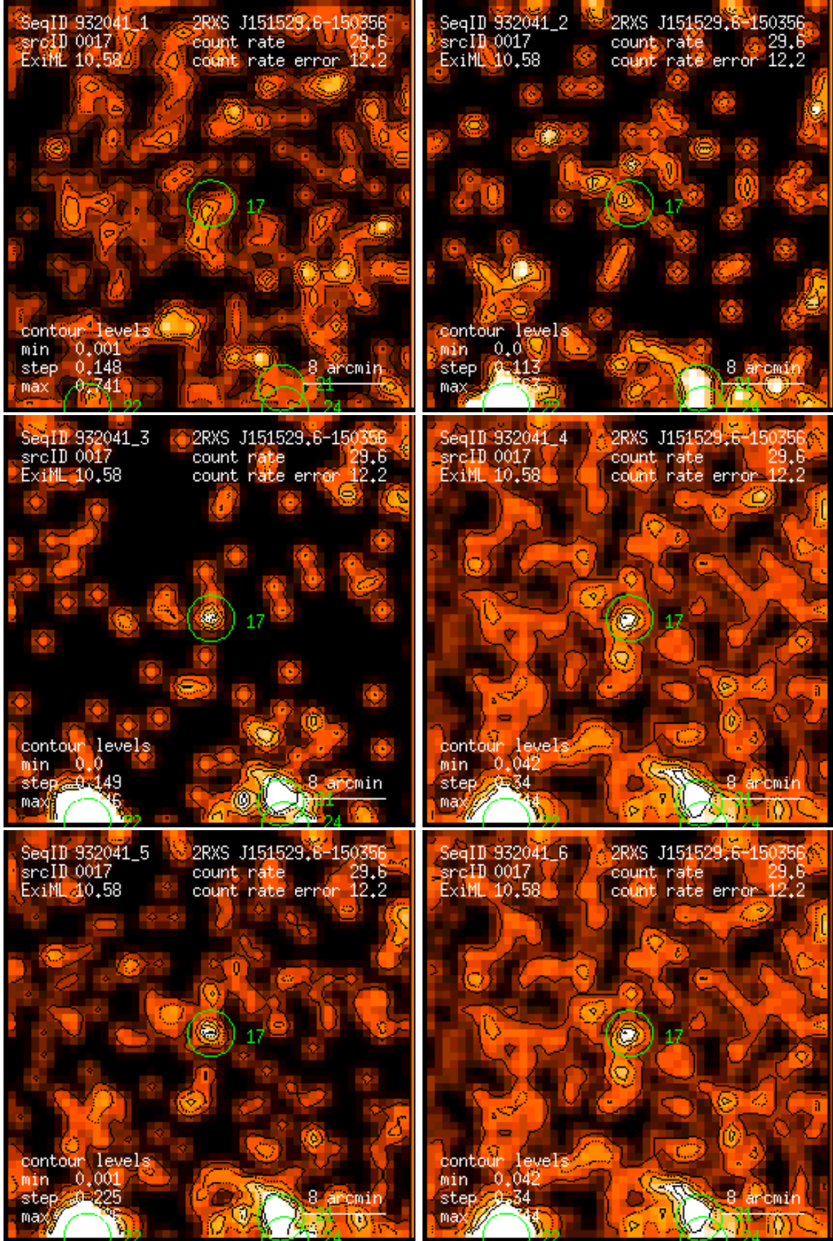
Figure 17: RASS 932041: detection 0017: band rate images, Gaussian filter: (1) PSPC channels 11 – 41, (2) 52 – 90, (3) 91 – 201, (4) 11 – 235, (5) 52 – 201, (6) 11 – 201. Broad band rates in counts/ks. Band rate contour levels in counts/ks/arcmin 2 .
