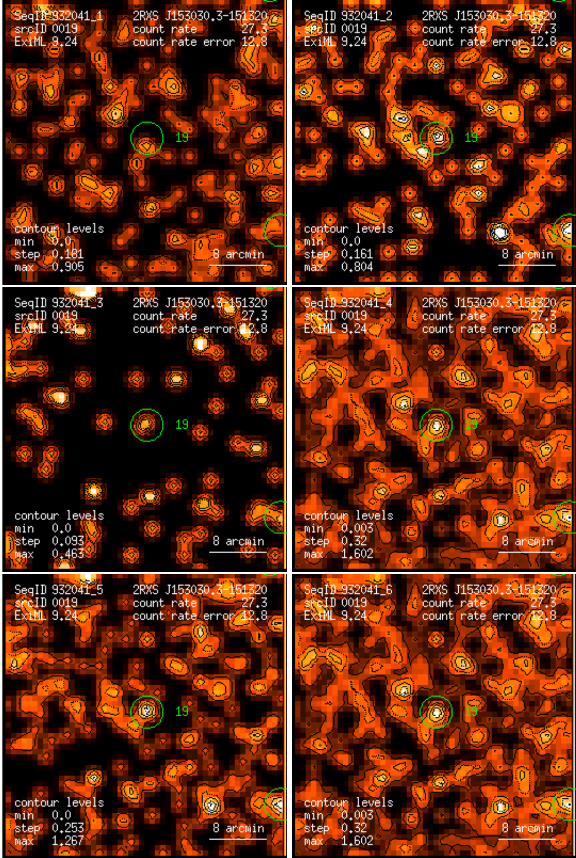
Figure 19: RASS 932041: detection 0019: band rate images, Gaussian filter: (1) PSPC channels 11 – 41, (2) 52 – 90, (3) 91 – 201, (4) 11 – 235, (5) 52 – 201, (6) 11 – 201. Broad band rates in counts/ks. Band rate contour levels in counts/ks/arcmin 2 .
