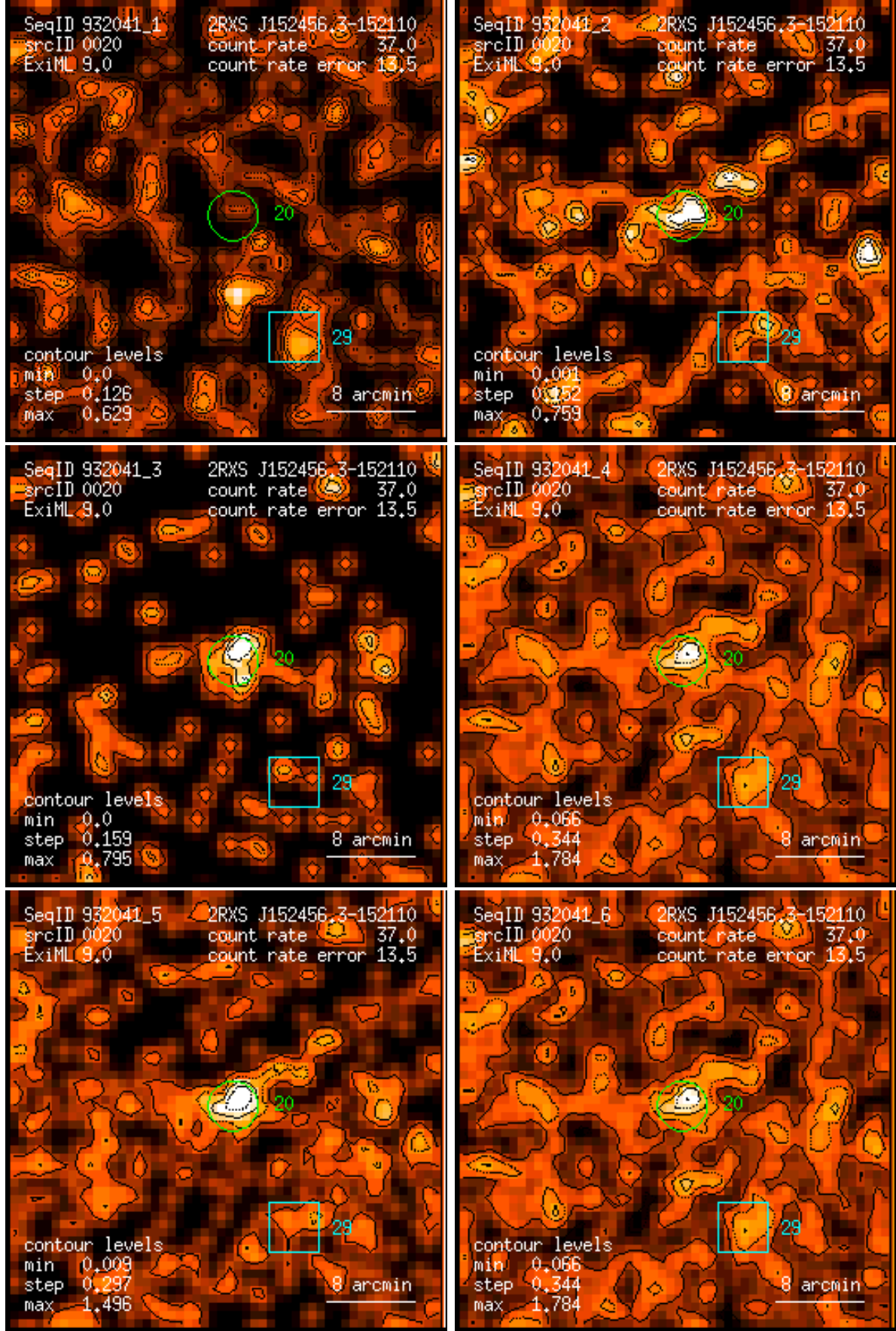
Figure 20: RASS 932041: detection 0020: band rate images, Gaussian filter: (1) PSPC channels 11 – 41, (2) 52 – 90, (3) 91 – 201, (4) 11 – 235, (5) 52 – 201, (6) 11 – 201. Broad band rates in counts/ks. Band rate contour levels in counts/ks/arcmin 2 .
