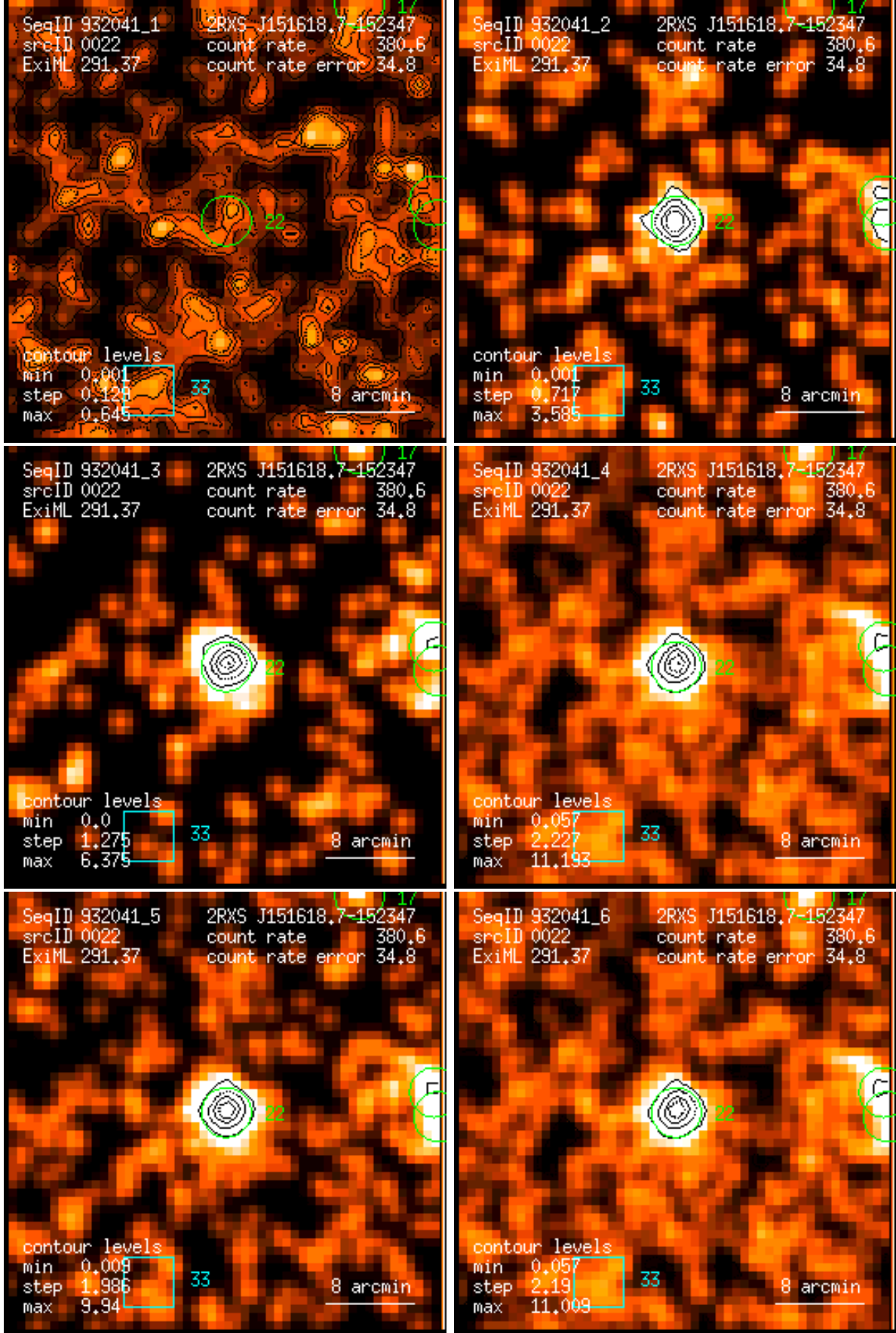
Figure 22: RASS 932041: detection 0022: band rate images, Gaussian filter: (1) PSPC channels 11 – 41, (2) 52 – 90, (3) 91 – 201, (4) 11 – 235, (5) 52 – 201, (6) 11 – 201. Broad band rates in counts/ks. Band rate contour levels in counts/ks/arcmin 2 .
