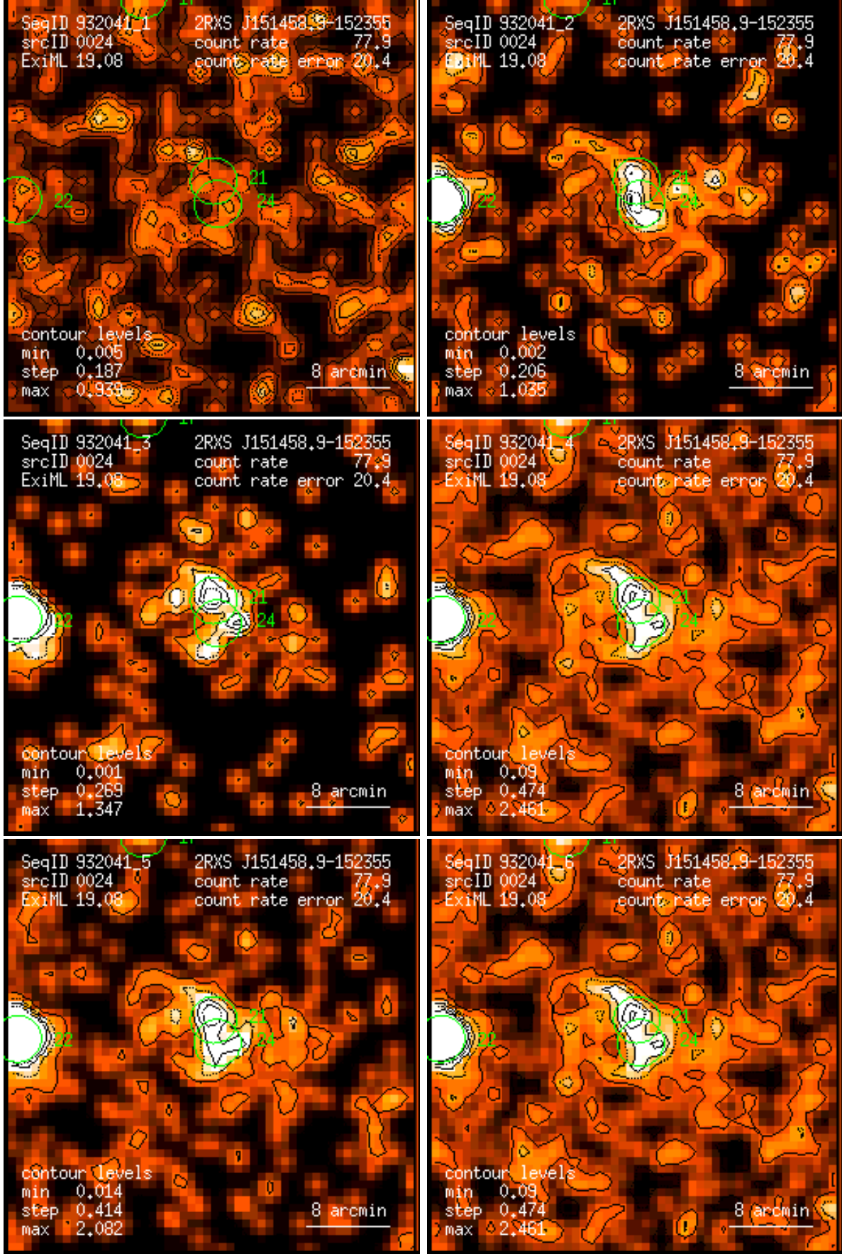
Figure 24: RASS 932041: detection 0024: band rate images, Gaussian filter: (1) PSPC channels 11 – 41, (2) 52 – 90, (3) 91 – 201, (4) 11 – 235, (5) 52 – 201, (6) 11 – 201. Broad band rates in counts/ks. Band rate contour levels in counts/ks/arcmin 2 .
