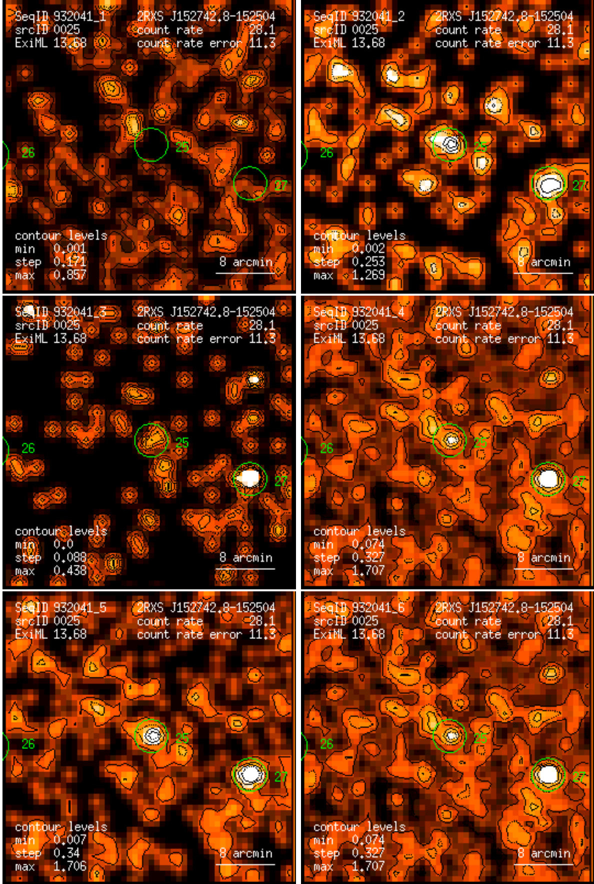
Figure 25: RASS 932041: detection 0025: band rate images, Gaussian filter: (1) PSPC channels 11 – 41, (2) 52 – 90, (3) 91 – 201, (4) 11 – 235, (5) 52 – 201, (6) 11 – 201. Broad band rates in counts/ks. Band rate contour levels in counts/ks/arcmin 2 .
