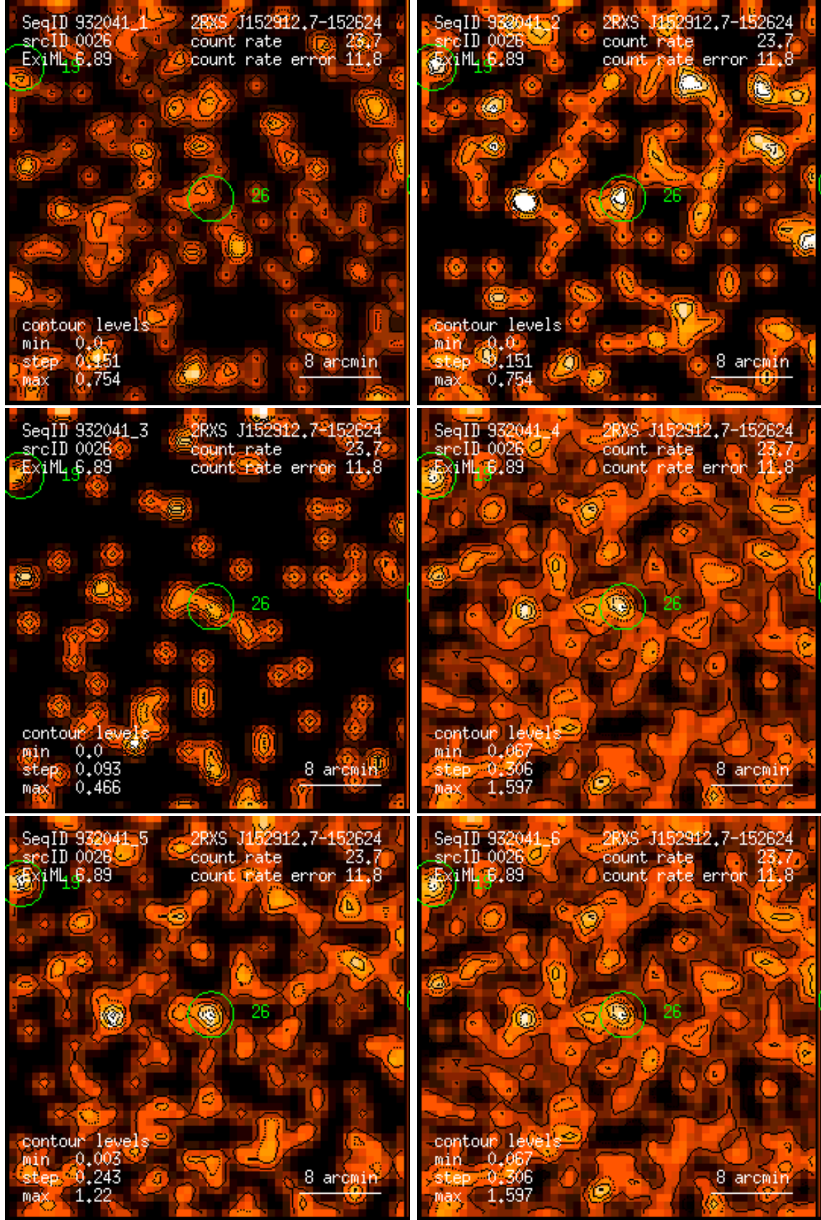
Figure 26: RASS 932041: detection 0026: band rate images, Gaussian filter: (1) PSPC channels 11 – 41, (2) 52 – 90, (3) 91 – 201, (4) 11 – 235, (5) 52 – 201, (6) 11 – 201. Broad band rates in counts/ks. Band rate contour levels in counts/ks/arcmin 2 .
