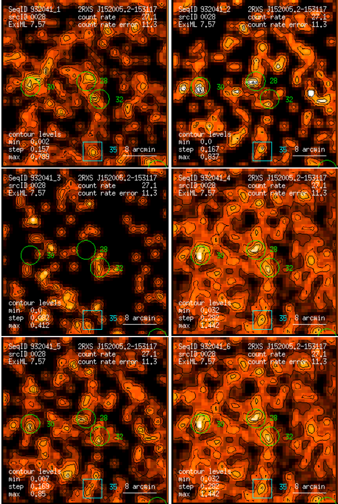
Figure 28: RASS 932041: detection 0028: band rate images, Gaussian filter: (1) PSPC channels 11 – 41, (2) 52 – 90, (3) 91 – 201, (4) 11 – 235, (5) 52 – 201, (6) 11 – 201. Broad band rates in counts/ks. Band rate contour levels in counts/ks/arcmin 2 .
