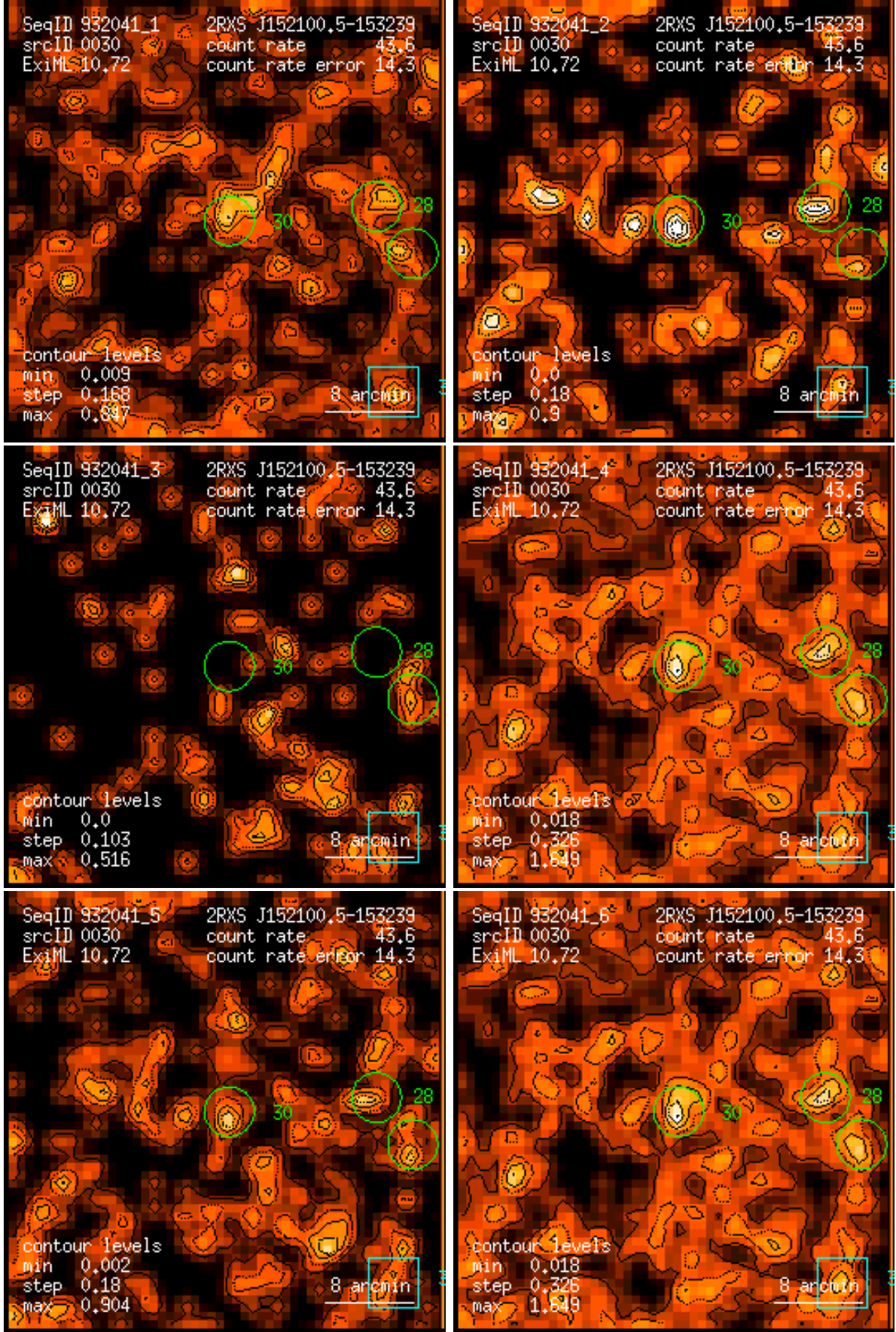
Figure 30: RASS 932041: detection 0030: band rate images, Gaussian filter: (1) PSPC channels 11 – 41, (2) 52 – 90, (3) 91 – 201, (4) 11 – 235, (5) 52 – 201, (6) 11 – 201. Broad band rates in counts/ks. Band rate contour levels in counts/ks/arcmin 2 .
