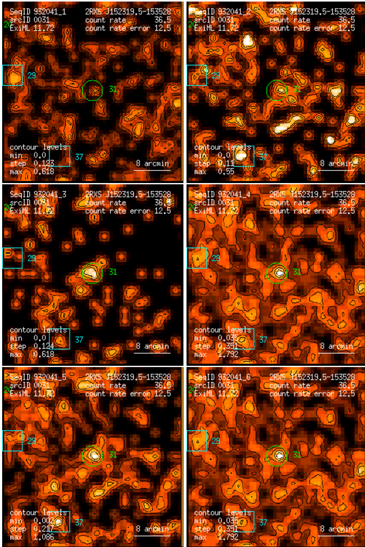
Figure 31: RASS 932041: detection 0031: band rate images, Gaussian filter: (1) PSPC channels 11 – 41, (2) 52 – 90, (3) 91 – 201, (4) 11 – 235, (5) 52 – 201, (6) 11 – 201. Broad band rates in counts/ks. Band rate contour levels in counts/ks/arcmin 2 .
