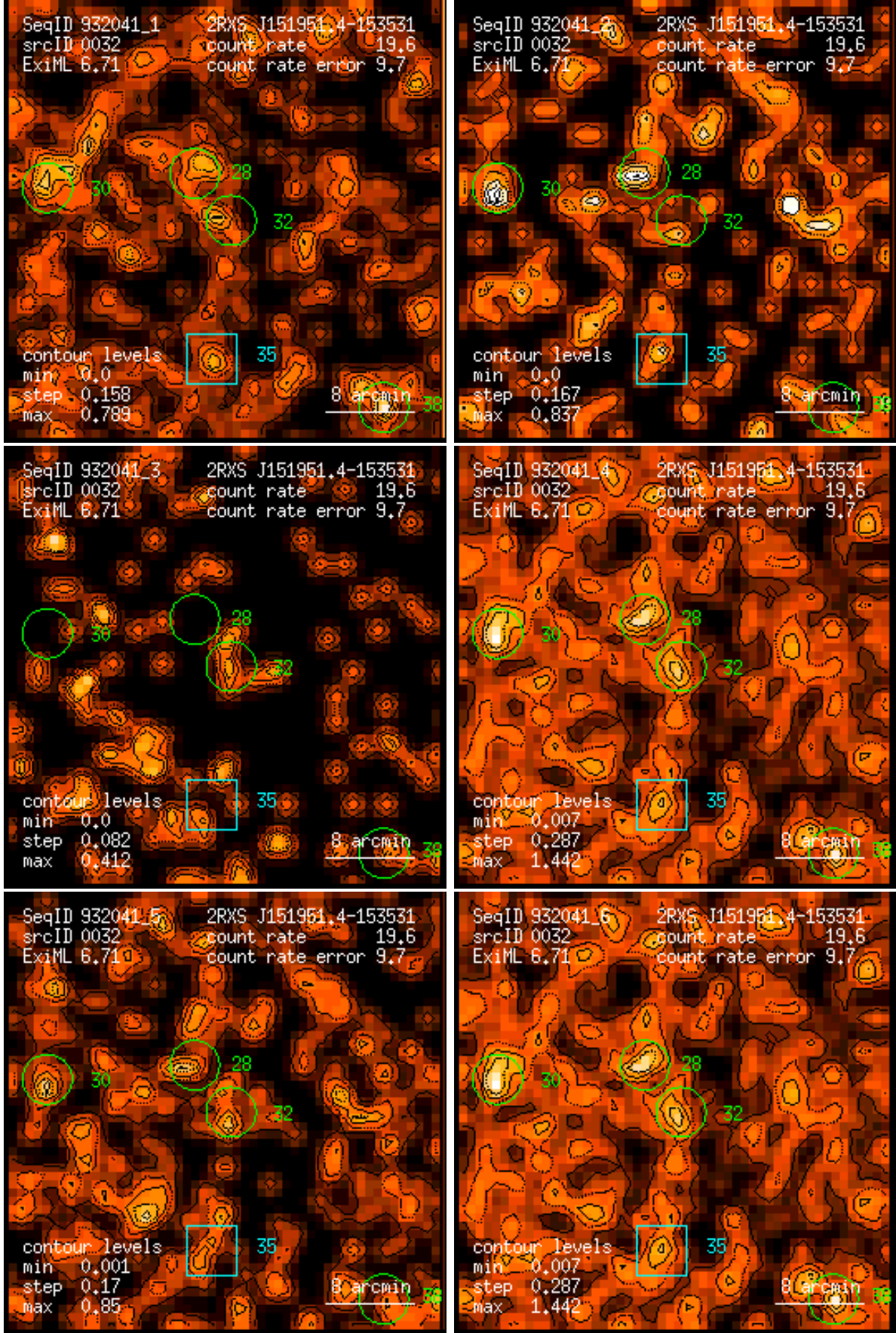
Figure 32: RASS 932041: detection 0032: band rate images, Gaussian filter: (1) PSPC channels 11 – 41, (2) 52 – 90, (3) 91 – 201, (4) 11 – 235, (5) 52 – 201, (6) 11 – 201. Broad band rates in counts/ks. Band rate contour levels in counts/ks/arcmin 2 .
