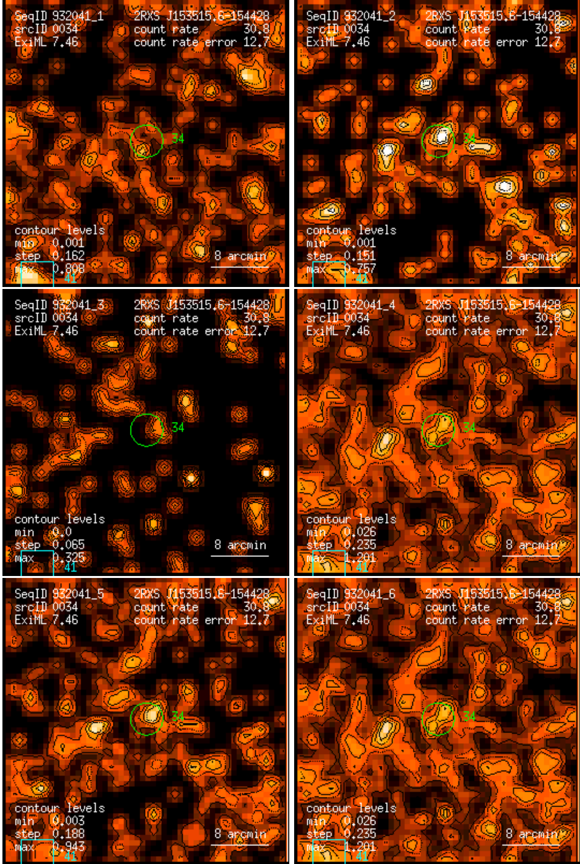
Figure 34: RASS 932041: detection 0034: band rate images, Gaussian filter: (1) PSPC channels 11 – 41, (2) 52 – 90, (3) 91 – 201, (4) 11 – 235, (5) 52 – 201, (6) 11 – 201. Broad band rates in counts/ks. Band rate contour levels in counts/ks/arcmin 2 .
