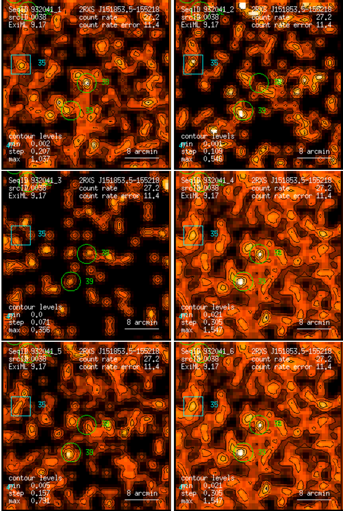
Figure 38: RASS 932041: detection 0038: band rate images, Gaussian filter: (1) PSPC channels 11 – 41, (2) 52 – 90, (3) 91 – 201, (4) 11 – 235, (5) 52 – 201, (6) 11 – 201. Broad band rates in counts/ks. Band rate contour levels in counts/ks/arcmin 2 .
