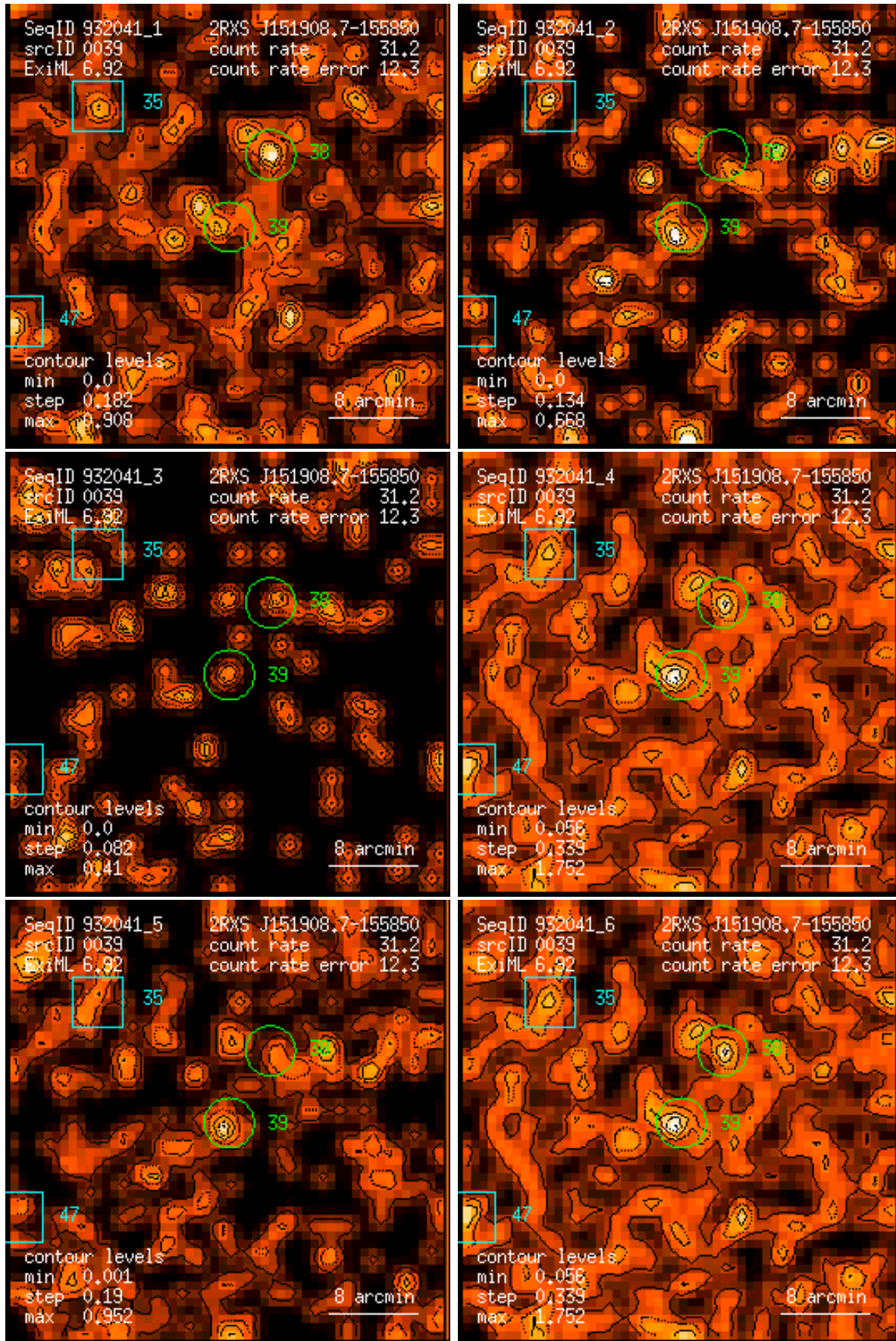
Figure 39: RASS 932041: detection 0039: band rate images, Gaussian filter: (1) PSPC channels 11 – 41, (2) 52 – 90, (3) 91 – 201, (4) 11 – 235, (5) 52 – 201, (6) 11 – 201. Broad band rates in counts/ks. Band rate contour levels in counts/ks/arcmin 2 .
