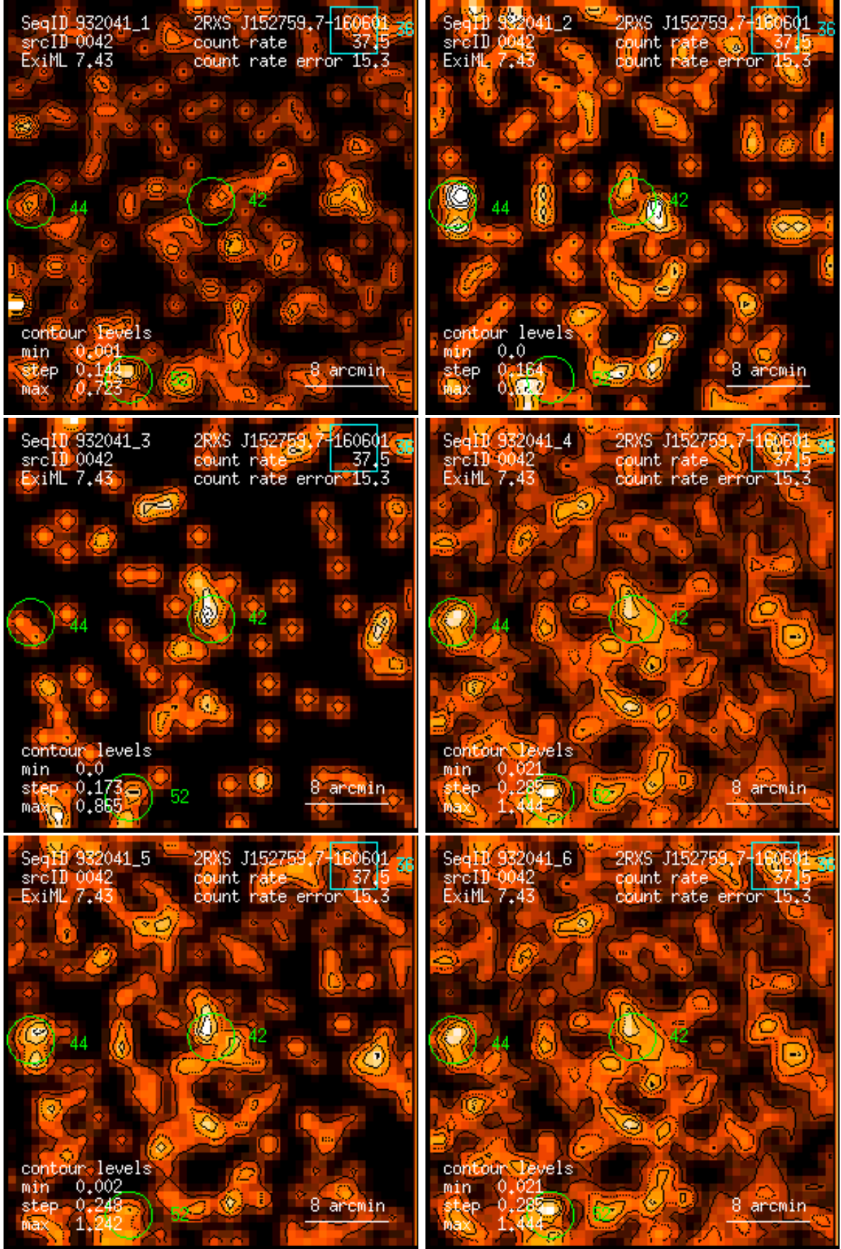
Figure 42: RASS 932041: detection 0042: band rate images, Gaussian filter: (1) PSPC channels 11 – 41, (2) 52 – 90, (3) 91 – 201, (4) 11 – 235, (5) 52 – 201, (6) 11 – 201. Broad band rates in counts/ks. Band rate contour levels in counts/ks/arcmin 2 .
