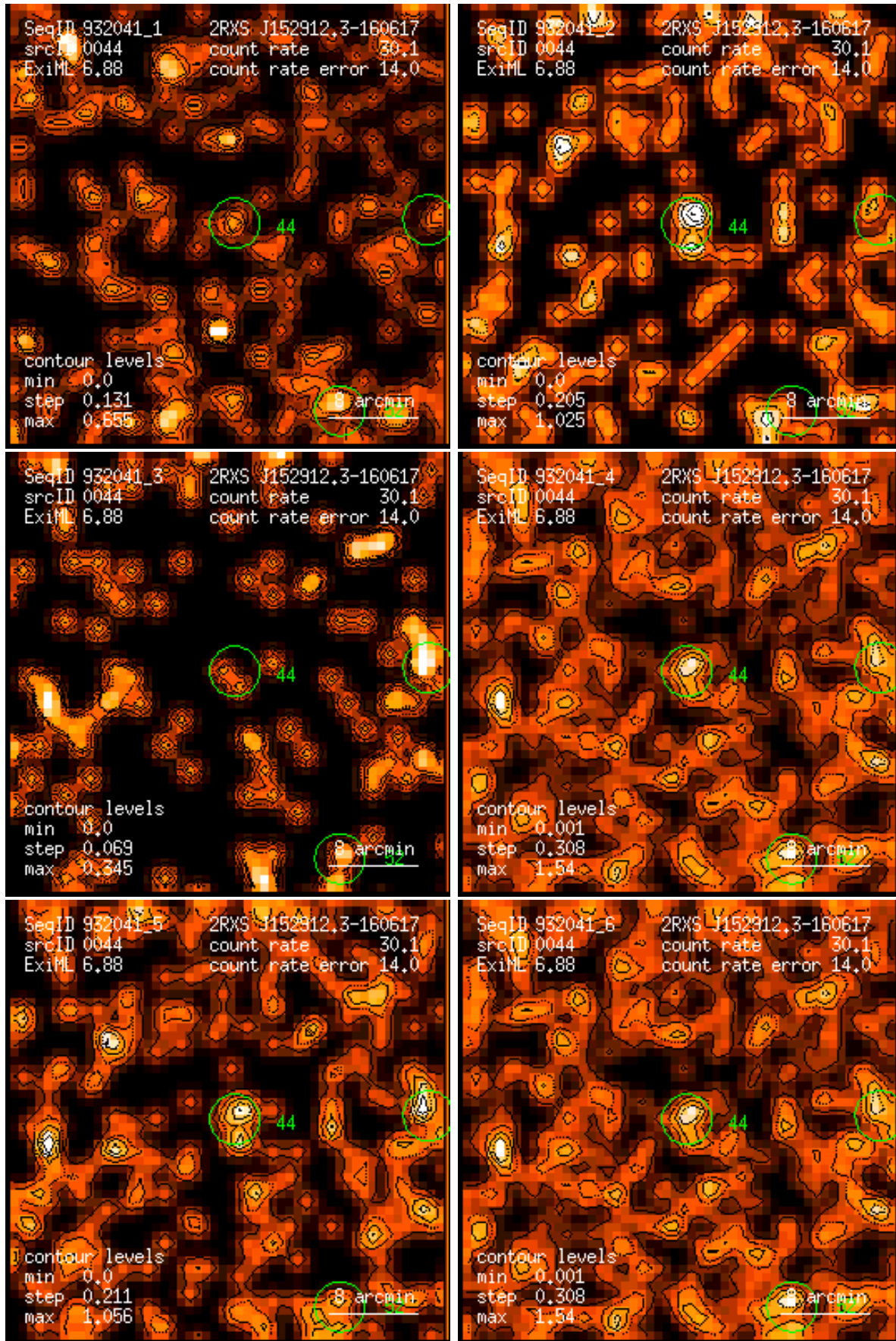
Figure 44: RASS 932041: detection 0044: band rate images, Gaussian filter: (1) PSPC channels 11 – 41, (2) 52 – 90, (3) 91 – 201, (4) 11 – 235, (5) 52 – 201, (6) 11 – 201. Broad band rates in counts/ks. Band rate contour levels in counts/ks/arcmin 2 .
