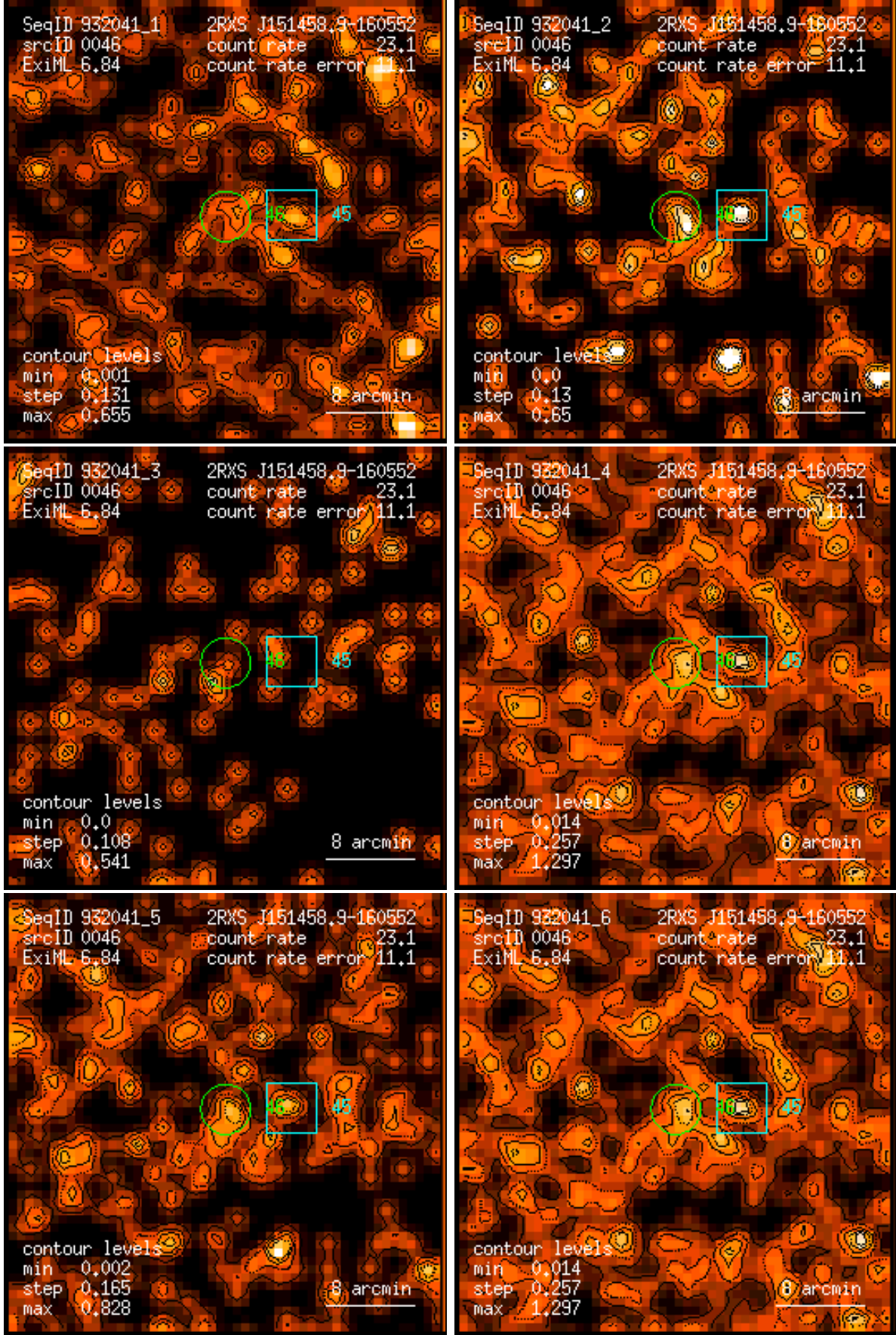
Figure 46: RASS 932041: detection 0046: band rate images, Gaussian filter: (1) PSPC channels 11 – 41, (2) 52 – 90, (3) 91 – 201, (4) 11 – 235, (5) 52 – 201, (6) 11 – 201. Broad band rates in counts/ks. Band rate contour levels in counts/ks/arcmin 2 .
