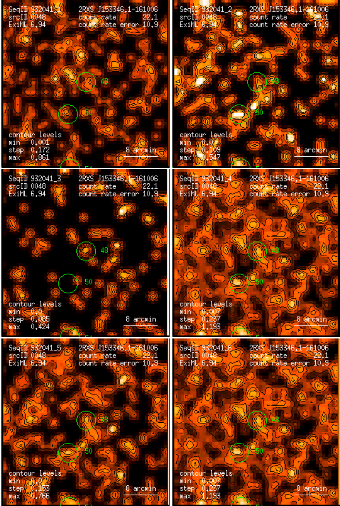
Figure 48: RASS 932041: detection 0048: band rate images, Gaussian filter: (1) PSPC channels 11 – 41, (2) 52 – 90, (3) 91 – 201, (4) 11 – 235, (5) 52 – 201, (6) 11 – 201. Broad band rates in counts/ks. Band rate contour levels in counts/ks/arcmin 2 .
