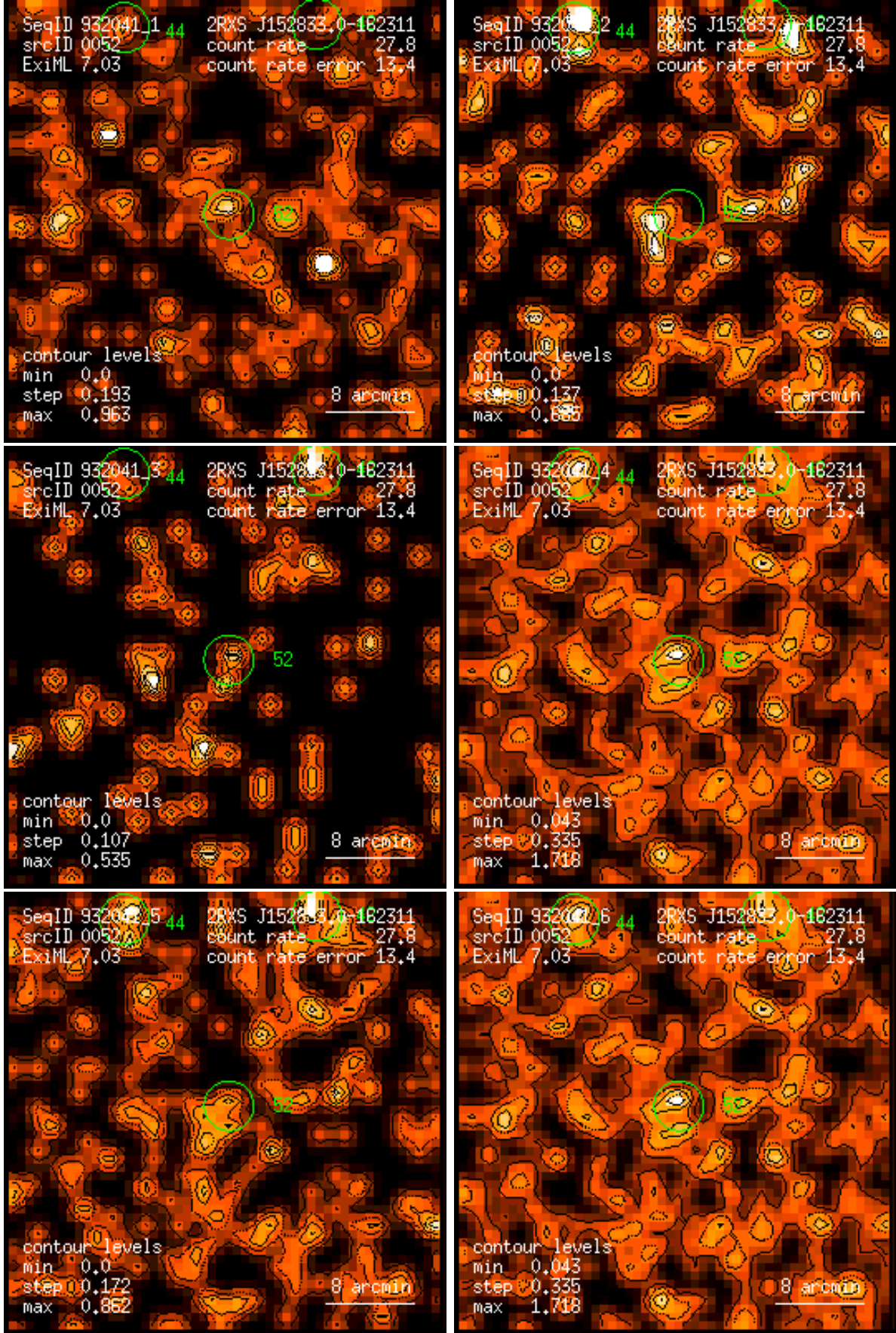
Figure 52: RASS 932041: detection 0052: band rate images, Gaussian filter: (1) PSPC channels 11 – 41, (2) 52 – 90, (3) 91 – 201, (4) 11 – 235, (5) 52 – 201, (6) 11 – 201. Broad band rates in counts/ks. Band rate contour levels in counts/ks/arcmin 2 .
