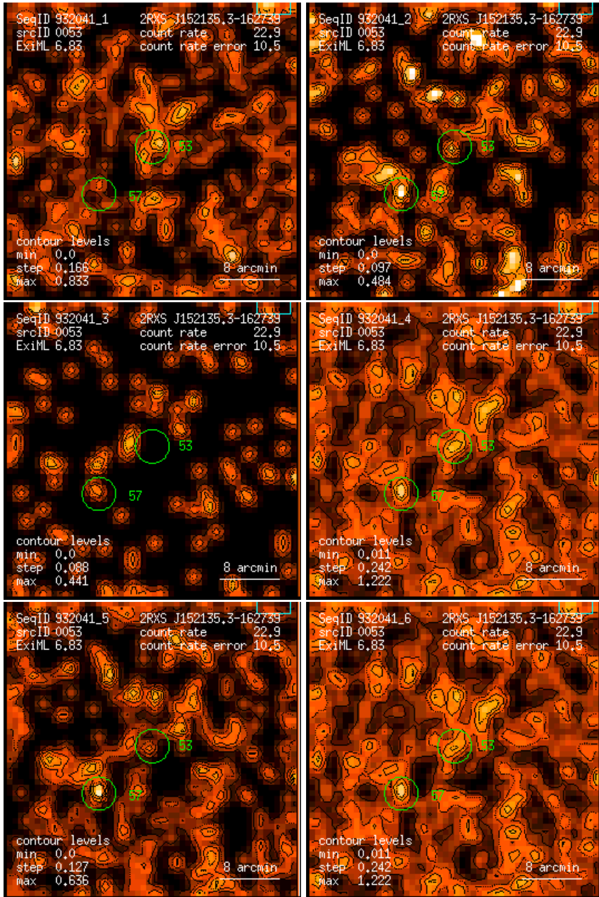
Figure 53: RASS 932041: detection 0053: band rate images, Gaussian filter: (1) PSPC channels 11 – 41, (2) 52 – 90, (3) 91 – 201, (4) 11 – 235, (5) 52 – 201, (6) 11 – 201. Broad band rates in counts/ks. Band rate contour levels in counts/ks/arcmin 2 .
