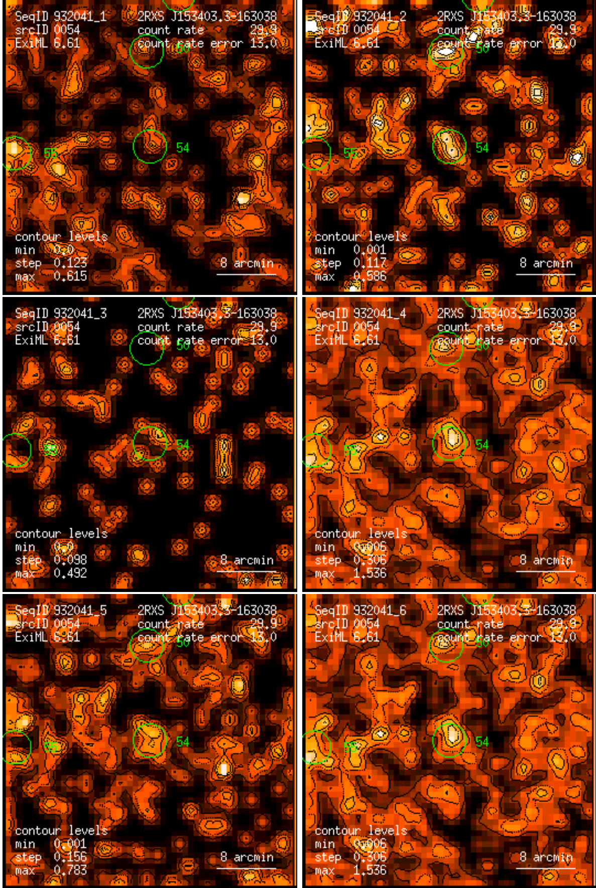
Figure 54: RASS 932041: detection 0054: band rate images, Gaussian filter: (1) PSPC channels 11 – 41, (2) 52 – 90, (3) 91 – 201, (4) 11 – 235, (5) 52 – 201, (6) 11 – 201. Broad band rates in counts/ks. Band rate contour levels in counts/ks/arcmin 2 .
