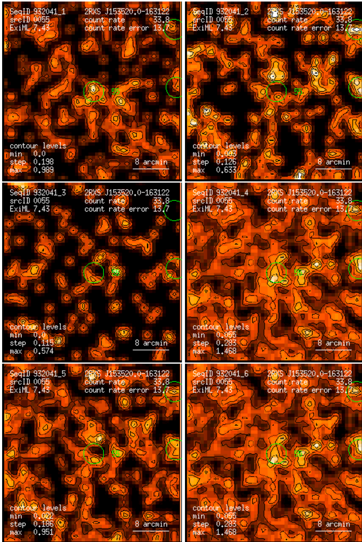
Figure 55: RASS 932041: detection 0055: band rate images, Gaussian filter: (1) PSPC channels 11 – 41, (2) 52 – 90, (3) 91 – 201, (4) 11 – 235, (5) 52 – 201, (6) 11 – 201. Broad band rates in counts/ks. Band rate contour levels in counts/ks/arcmin 2 .
