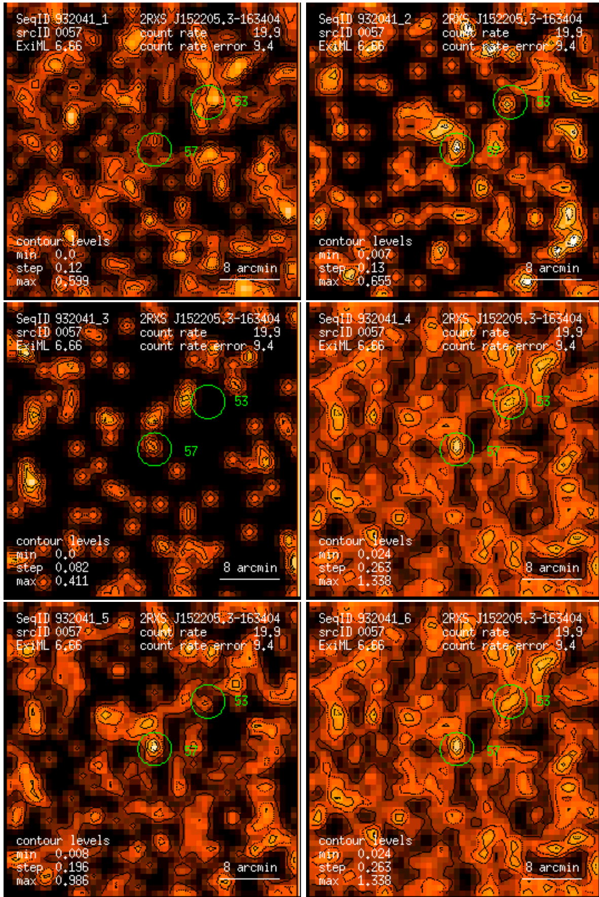
Figure 57: RASS 932041: detection 0057: band rate images, Gaussian filter: (1) PSPC channels 11 – 41, (2) 52 – 90, (3) 91 – 201, (4) 11 – 235, (5) 52 – 201, (6) 11 – 201. Broad band rates in counts/ks. Band rate contour levels in counts/ks/arcmin 2 .
