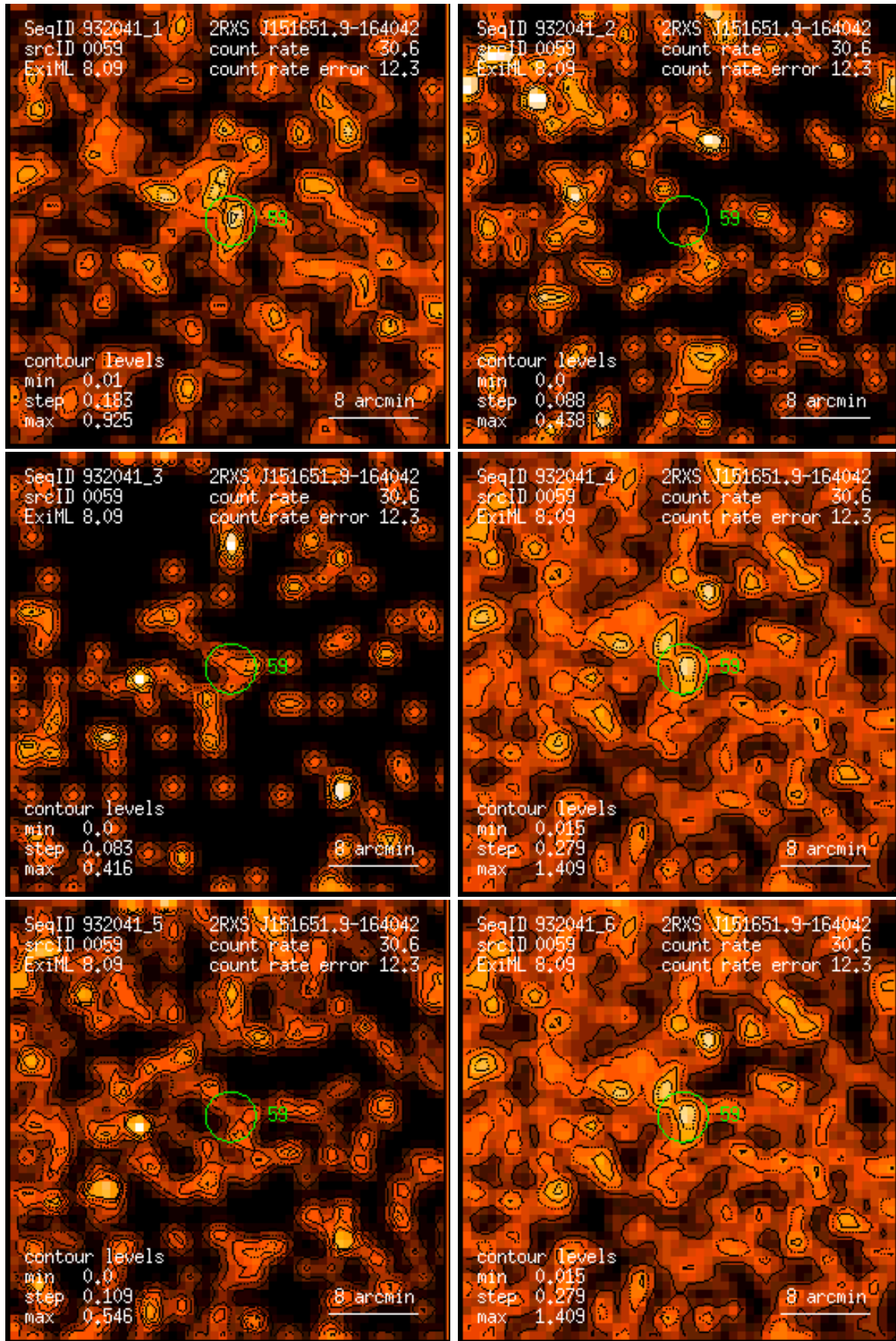
Figure 59: RASS 932041: detection 0059: band rate images, Gaussian filter: (1) PSPC channels 11 – 41, (2) 52 – 90, (3) 91 – 201, (4) 11 – 235, (5) 52 – 201, (6) 11 – 201. Broad band rates in counts/ks. Band rate contour levels in counts/ks/arcmin 2 .
