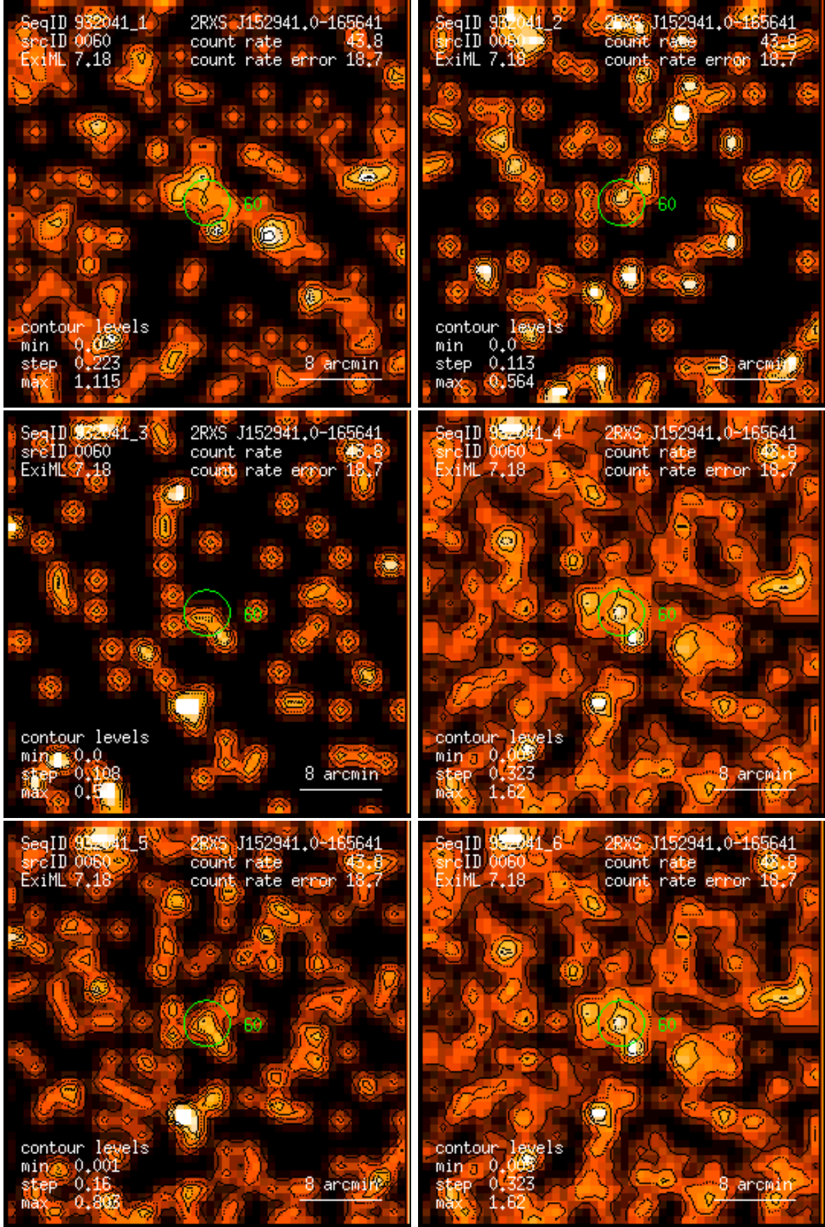
Figure 60: RASS 932041: detection 0060: band rate images, Gaussian filter: (1) PSPC channels 11 – 41, (2) 52 – 90, (3) 91 – 201, (4) 11 – 235, (5) 52 – 201, (6) 11 – 201. Broad band rates in counts/ks. Band rate contour levels in counts/ks/arcmin 2 .
