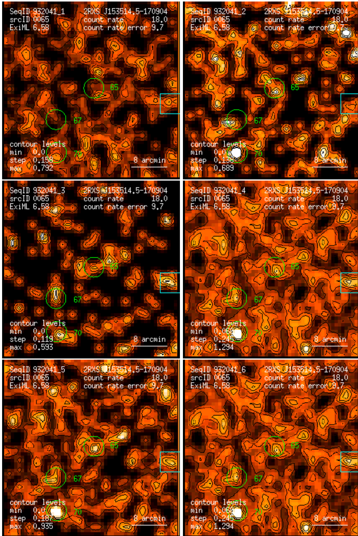
Figure 65: RASS 932041: detection 0065: band rate images, Gaussian filter: (1) PSPC channels 11 – 41, (2) 52 – 90, (3) 91 – 201, (4) 11 – 235, (5) 52 – 201, (6) 11 – 201. Broad band rates in counts/ks. Band rate contour levels in counts/ks/arcmin 2 .
