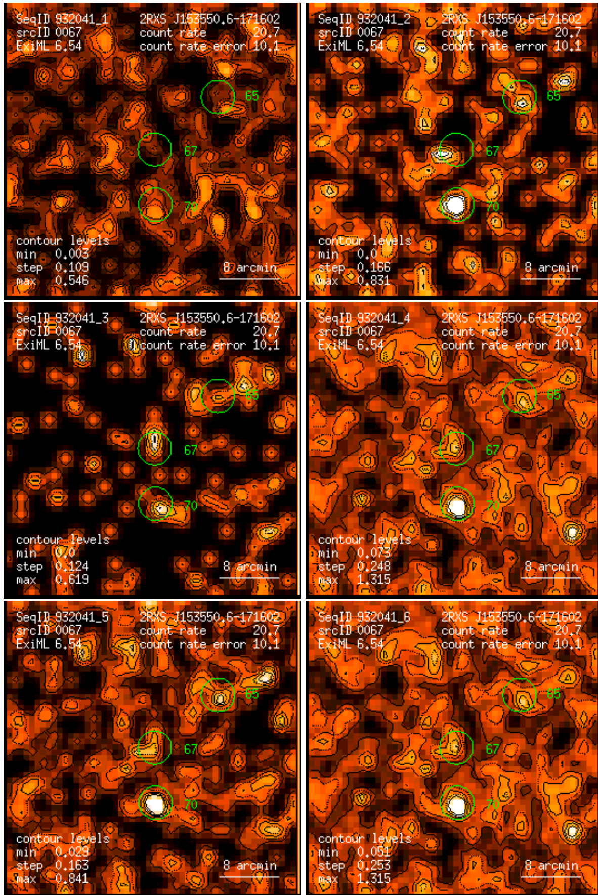
Figure 67: RASS 932041: detection 0067: band rate images, Gaussian filter: (1) PSPC channels 11 – 41, (2) 52 – 90, (3) 91 – 201, (4) 11 – 235, (5) 52 – 201, (6) 11 – 201. Broad band rates in counts/ks. Band rate contour levels in counts/ks/arcmin 2 .
