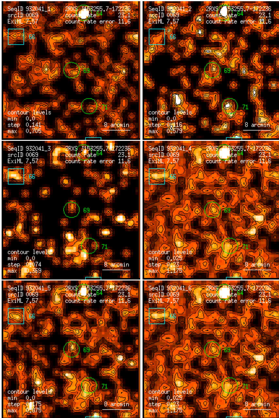
Figure 69: RASS 932041: detection 0069: band rate images, Gaussian filter: (1) PSPC channels 11 – 41, (2) 52 – 90, (3) 91 – 201, (4) 11 – 235, (5) 52 – 201, (6) 11 – 201. Broad band rates in counts/ks. Band rate contour levels in counts/ks/arcmin 2 .
