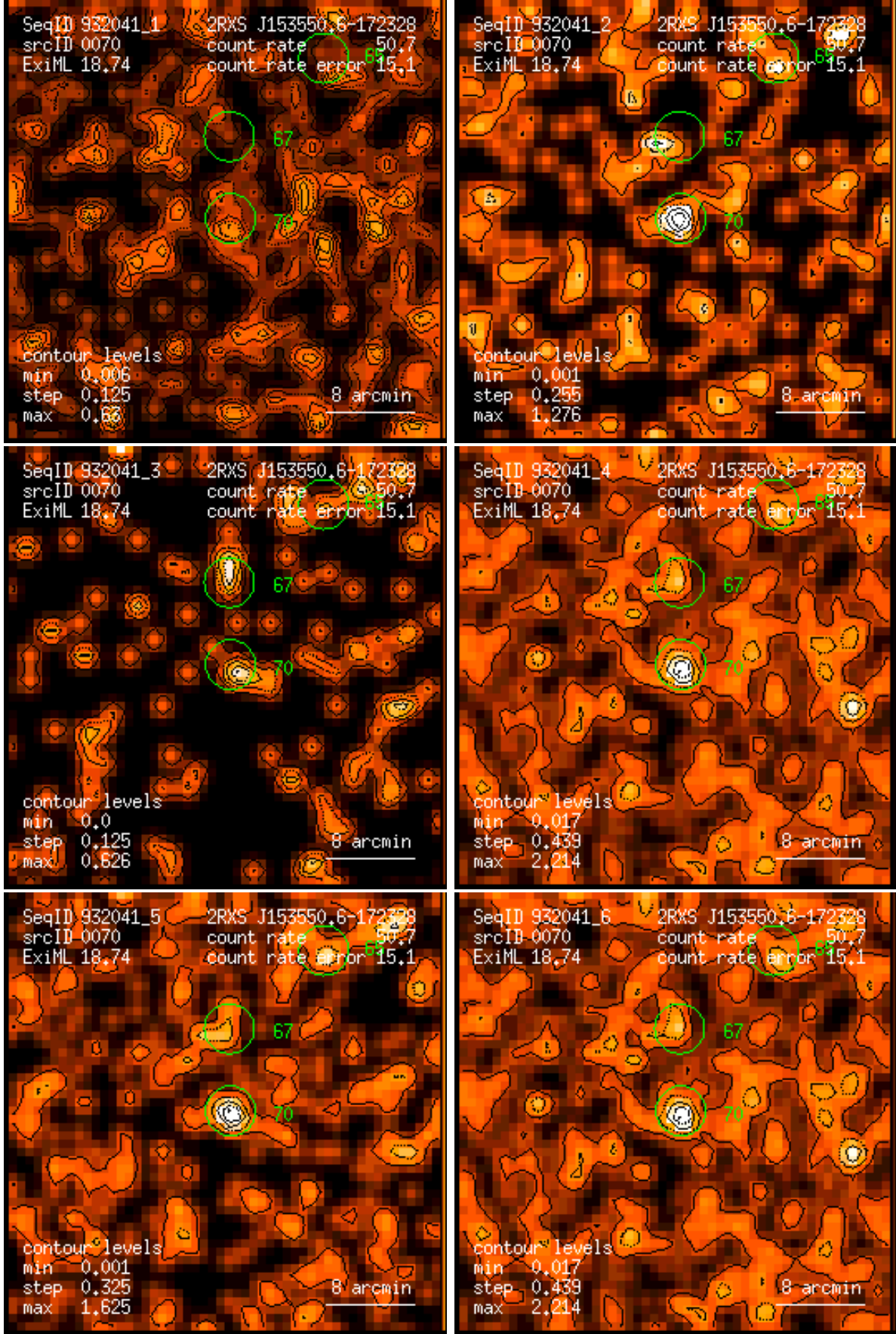
Figure 70: RASS 932041: detection 0070: band rate images, Gaussian filter: (1) PSPC channels 11 – 41, (2) 52 – 90, (3) 91 – 201, (4) 11 – 235, (5) 52 – 201, (6) 11 – 201. Broad band rates in counts/ks. Band rate contour levels in counts/ks/arcmin 2 .
