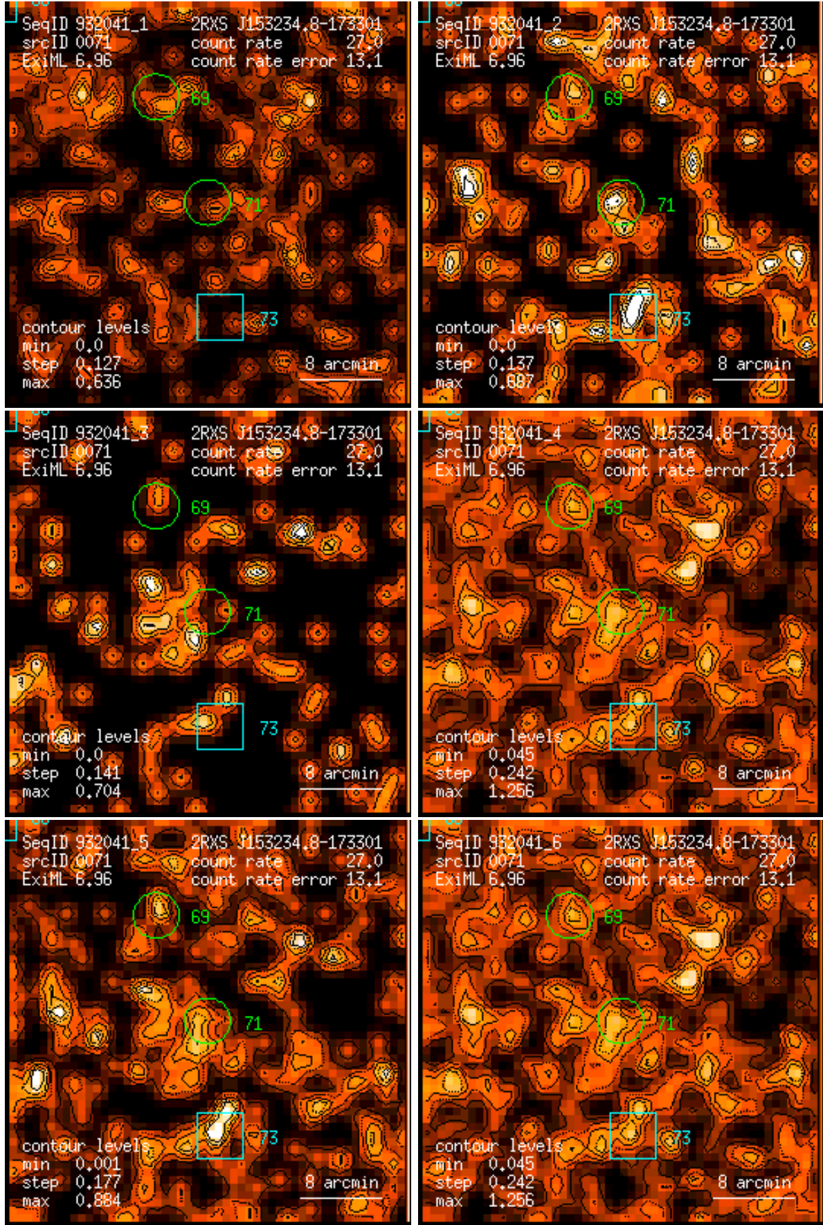
Figure 71: RASS 932041: detection 0071: band rate images, Gaussian filter: (1) PSPC channels 11 – 41, (2) 52 – 90, (3) 91 – 201, (4) 11 – 235, (5) 52 – 201, (6) 11 – 201. Broad band rates in counts/ks. Band rate contour levels in counts/ks/arcmin 2 .
