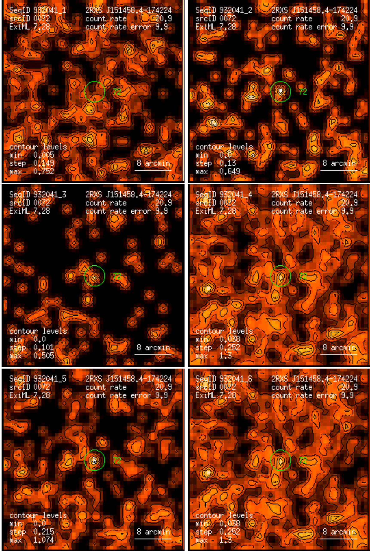
Figure 72: RASS 932041: detection 0072: band rate images, Gaussian filter: (1) PSPC channels 11 – 41, (2) 52 – 90, (3) 91 – 201, (4) 11 – 235, (5) 52 – 201, (6) 11 – 201. Broad band rates in counts/ks. Band rate contour levels in counts/ks/arcmin 2 .
