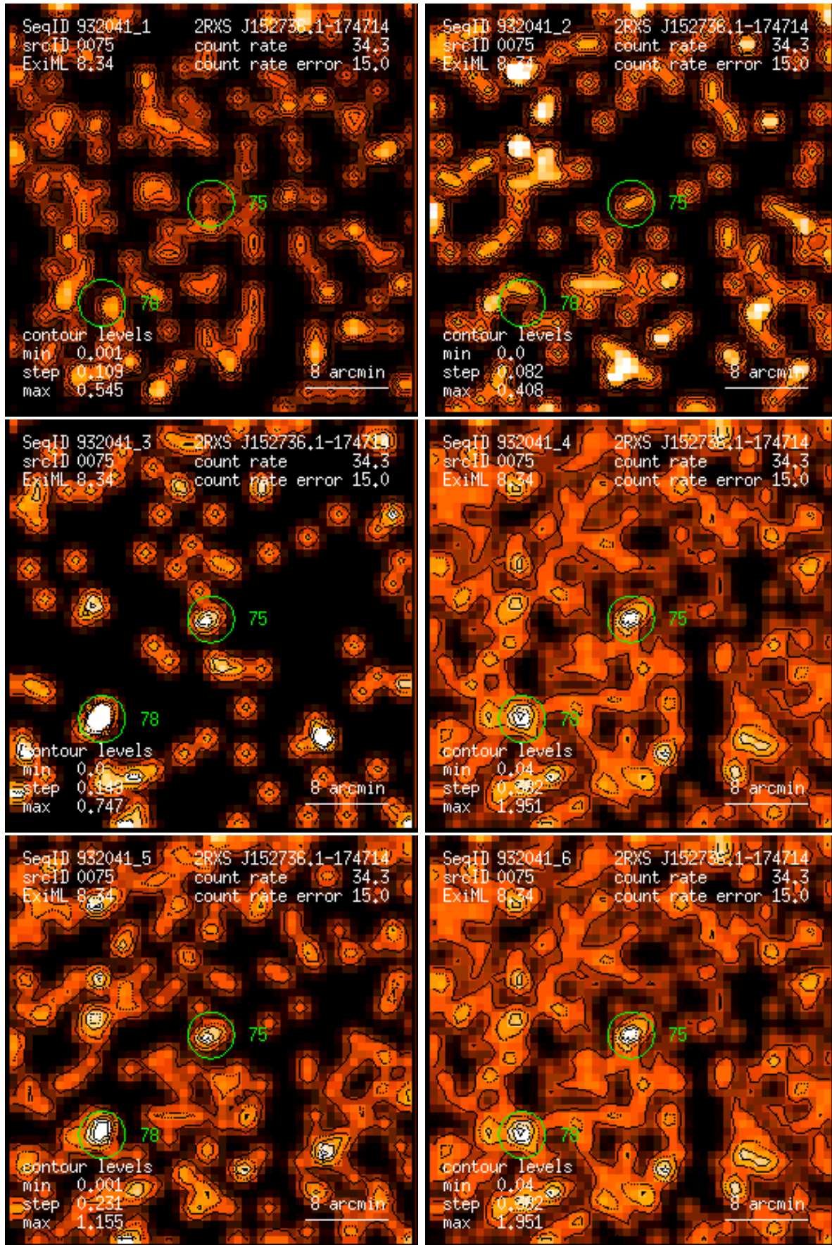
Figure 75: RASS 932041: detection 0075: band rate images, Gaussian filter: (1) PSPC channels 11 – 41, (2) 52 – 90, (3) 91 – 201, (4) 11 – 235, (5) 52 – 201, (6) 11 – 201. Broad band rates in counts/ks. Band rate contour levels in counts/ks/arcmin 2 .
